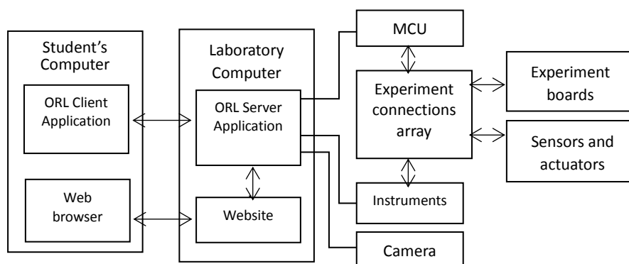
Figure 1 The ORL system architecture
