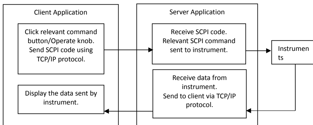
Figure 2 Instrument control architecture of the ORL system
