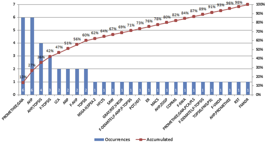
Figure 15. MCDM methods combined in analyzed papers.
