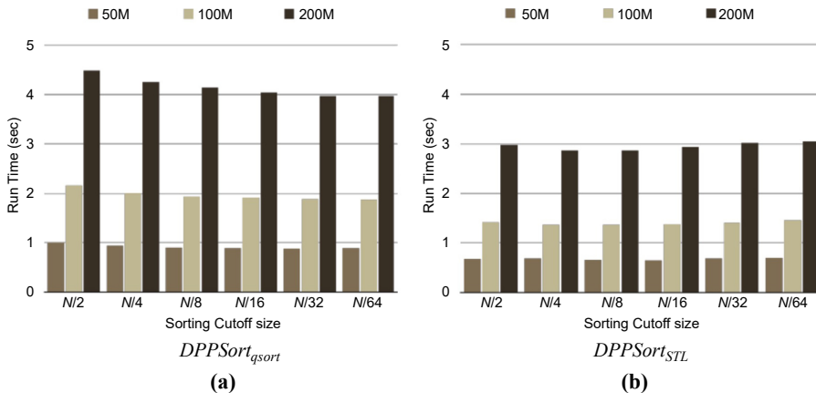
Figure 2. Run time of DPPSort_{qsort} in seconds vs Sorting cutoff size of various N ( M = 10^6 , Uint64 random)
