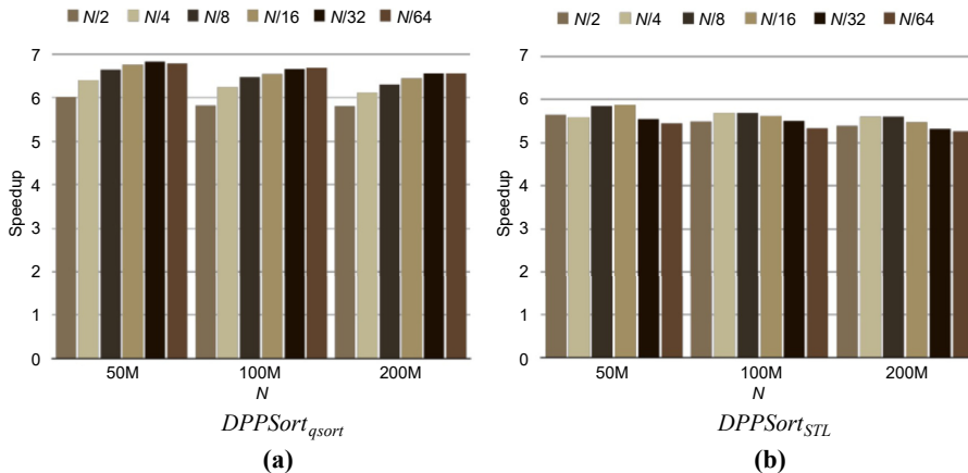
Figure 3. Speedup of DPPSort_{qsort} and DPPSort_{STL} vs N ( M = 10^6 , Uint64 Random) of various sorting cutoff size
