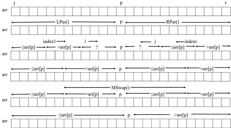
Figure 1. The illustration of DPPartition
