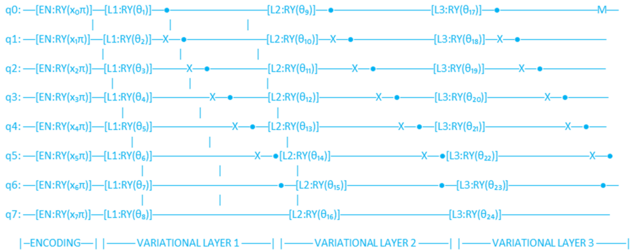
Figure 2. Schematic of the 8-qubit VQC architecture. The circuit comprises an encoding layer (EN) implementing angle encoding via R_Y(x_i \cdot \pi) gates, followed by three variational layers (L1, L2, L3), each containing parameterized R_Y(\theta) rotations and circular entanglement via CNOT gates (●—X connections). Measurement is performed on the first qubit (q0).
