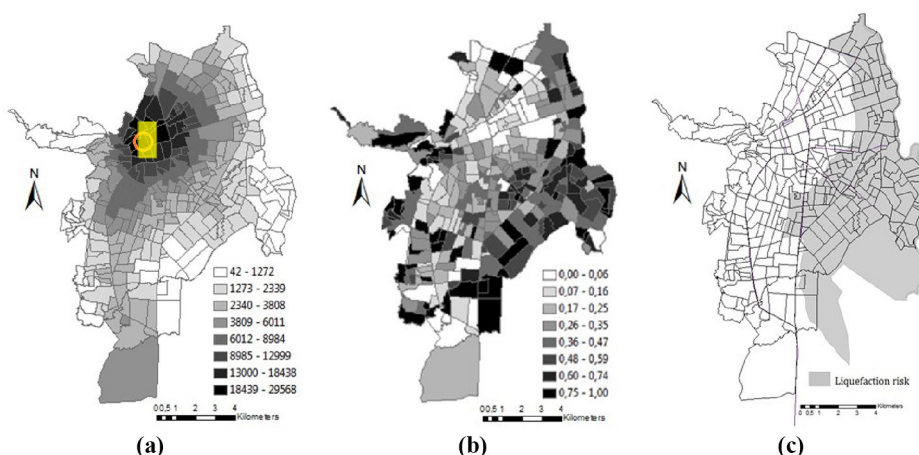
Figure 2. (a) Agglomeration, (b) informality share and (c) liquefaction risk
