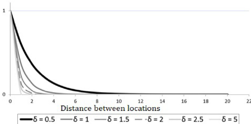
Figure 1. Weights as a function of the decay parameter \delta
