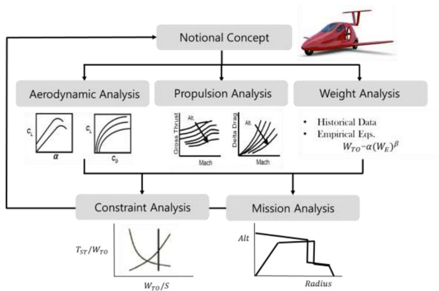
Figure 2 PAV sizing process
