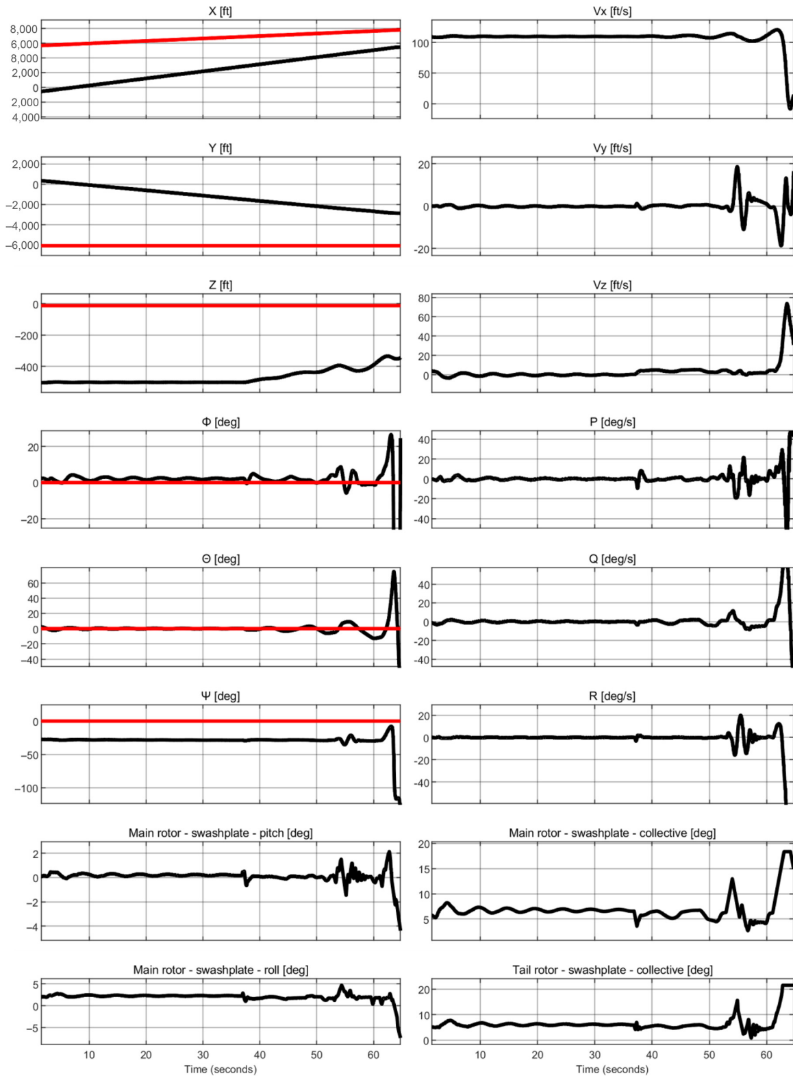
Figure 5 Case 3 – autopilot based on LQR, lack of information about pitch angle value
