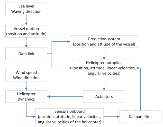
Figure 2 Information flow in the control system
