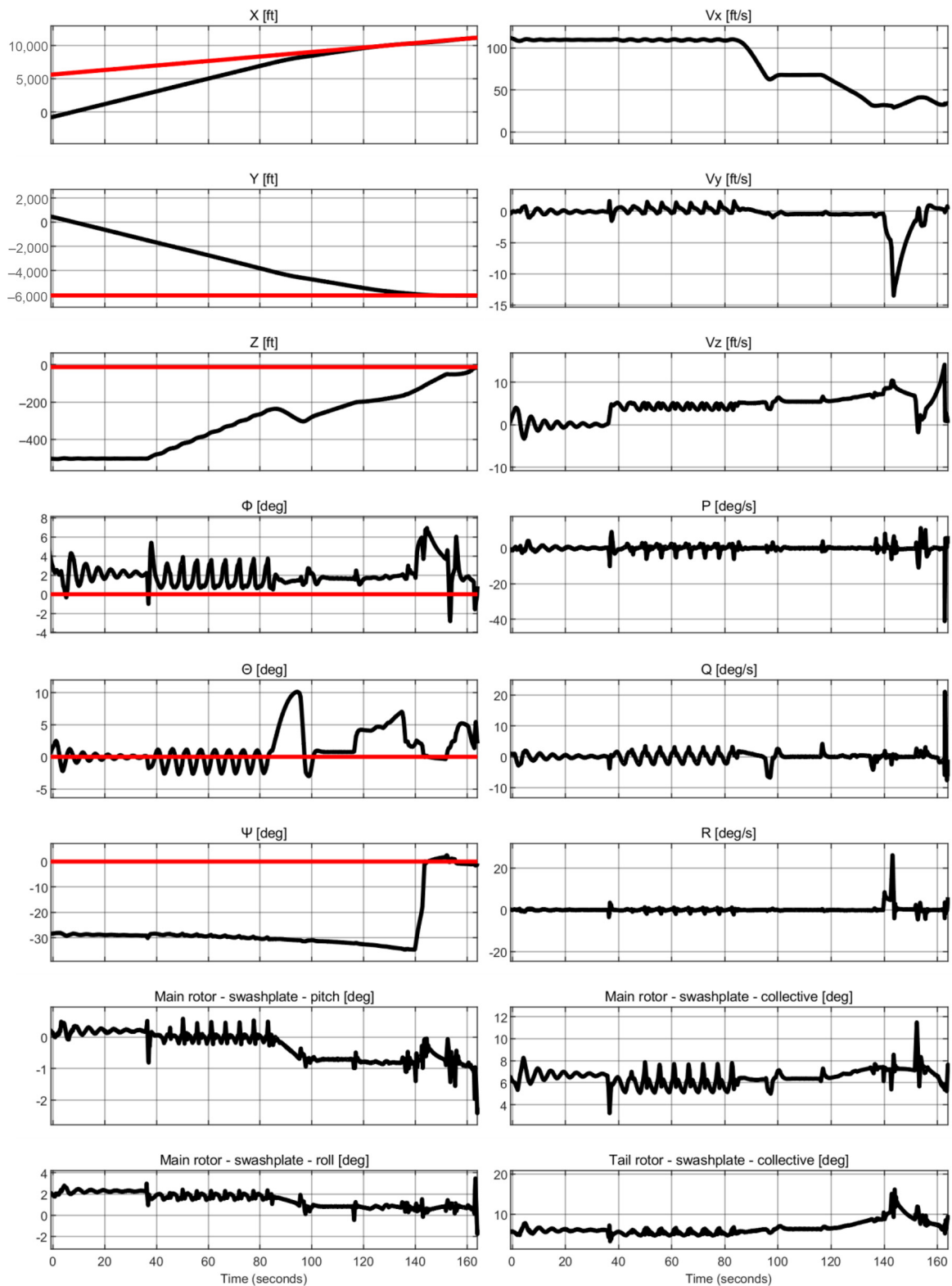
Figure 4 Case 2 – autopilot based on LQG, information about helicopter state variables constantly available
