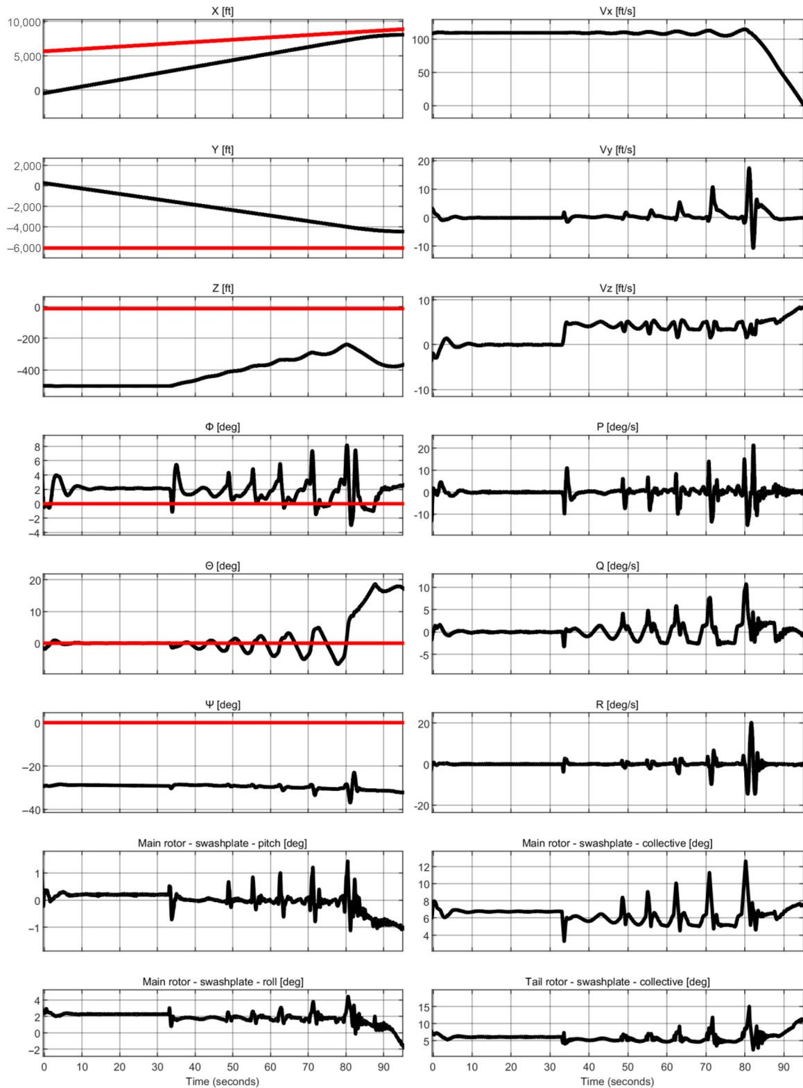
Figure 6 Case 4 – autopilot based on LQG, lack of information about pitch angle value
