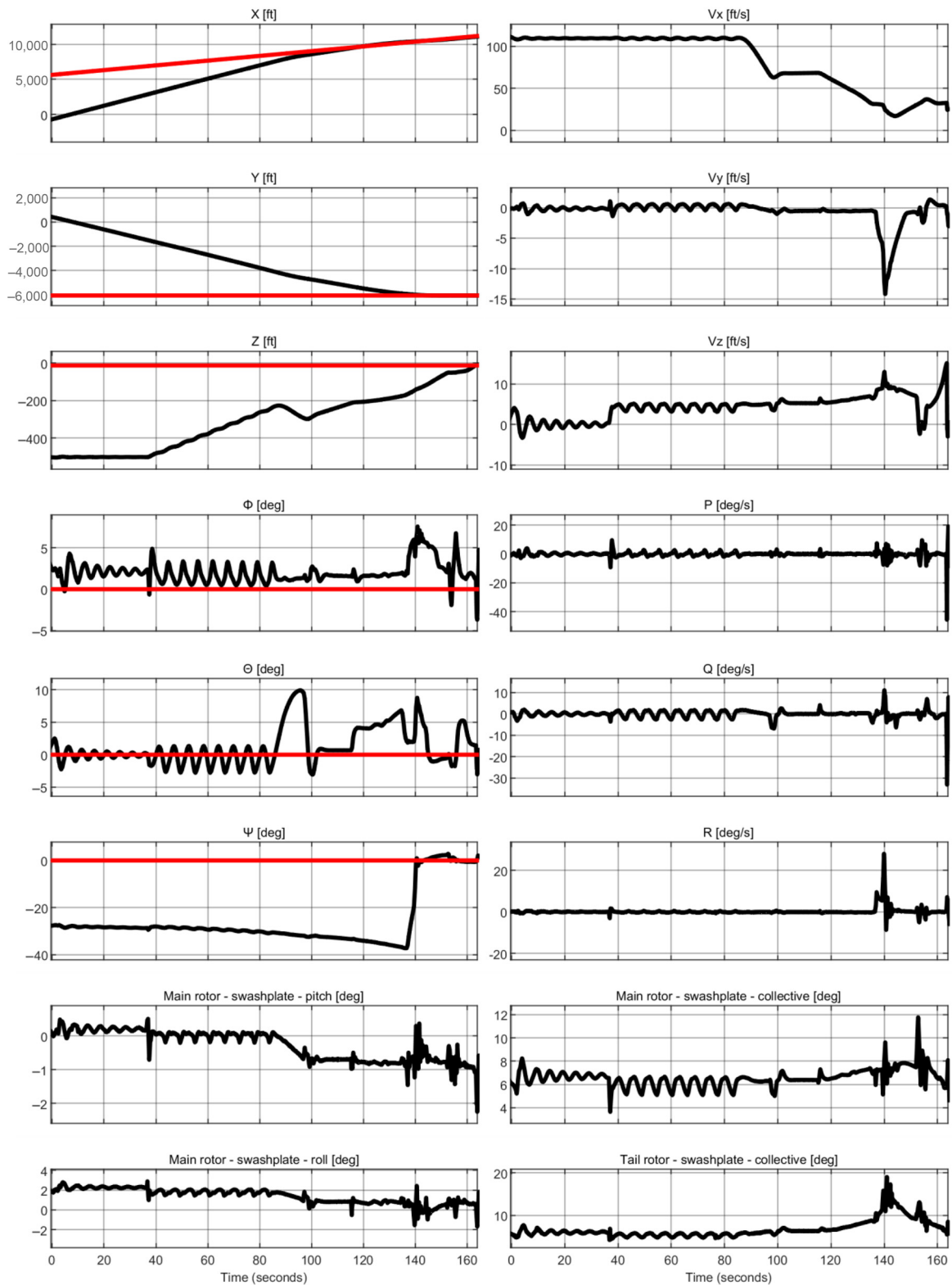
Figure 3 Case 1 – autopilot based on LQR, information about helicopter state variables constantly available
