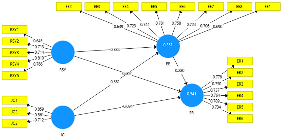
Figure 2. Measurement model
