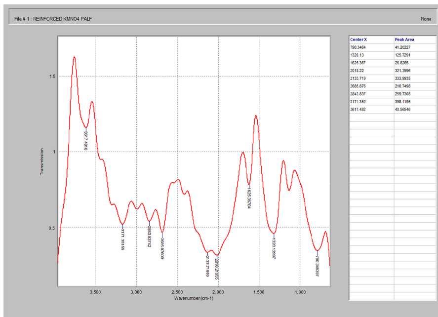
Figure 4. FTIR of permanganate treated PALF reinforced with TBR
