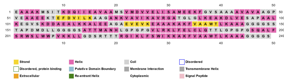
Figure 9. Secondary structure of multi-epitope vaccine (MEV). The alpha helix residues are pink, the coil residues are gray and the beta-strand is yellow
