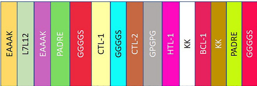
Figure 1. Visual representation of a sequence of epitopes and linkers used for polytope construct
