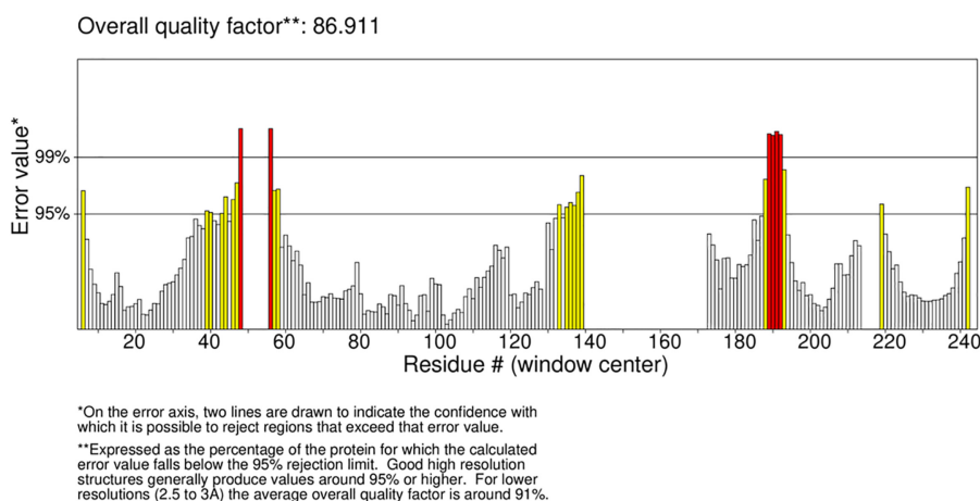
Figure 8. ERRAT predicted overall quality factor for structure analysis of the constructed model with a score of 86.911. The plot represents quality score along with error rates for the residues
