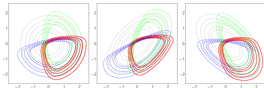
Figure 1. Contour plot of bivariate normal, SN and close SN distributions with various values of parameters
