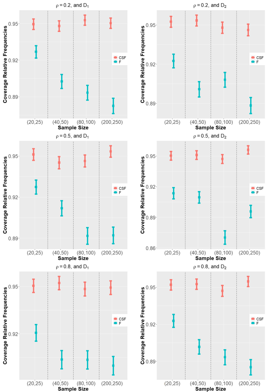
Figure 3. The confidence intervals of coverage relative frequencies at confidence level \alpha = 0.95 , red ones based on SN model and blue ones based on normal model with sample size (n_1, n_2) = (20, 25), (40, 50), (80, 100) and (200, 250) (from left to right in each figure), \rho = 0.2, 0.5 and 0.8 (in each row), and D_1 and D_2 (from left to right), respectively
