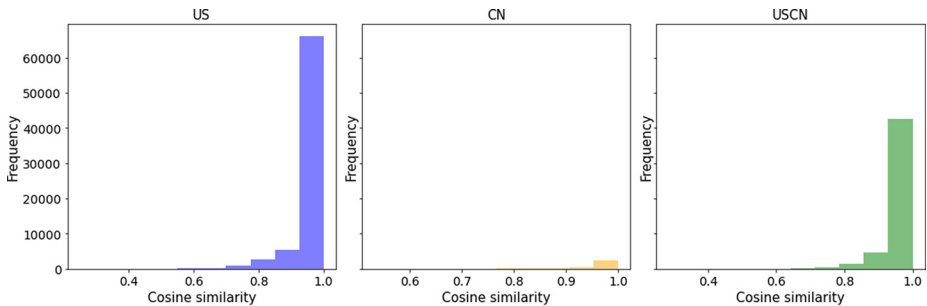
Figure 4. Histograms of cosine similarity between pairs within patent families
