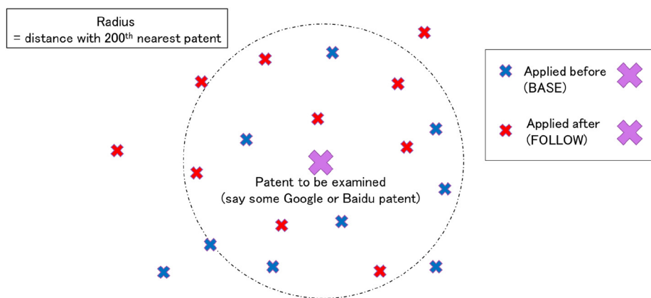
Figure 12. Graphical interpretation of NGT results
