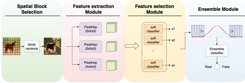
Figure 2: An overview of the proposed RGGID method.
