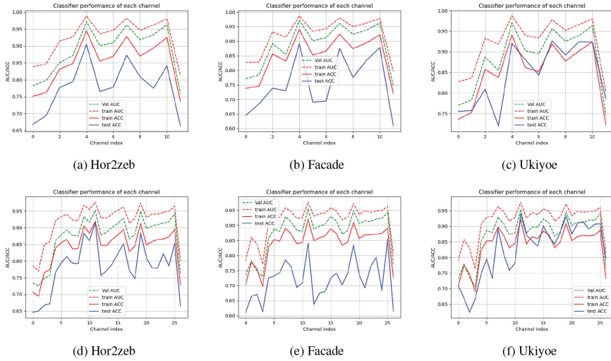
Figure 4: The detection performance on raw images of three exemplary categories, where the x -axis indicates the channel index. The x -value ranges from 0 to 11 in (a)–(c), in which a PixelHop of size 2 \times 2 \times 3 is used. The x -value ranges from 0 to 26 in (d)–(f), in which a PixelHop of size 3 \times 3 \times 3 is used. Each subfigure shows four performance curves: training AUC (red dashed line), training ACC (red line), validation AUC (green dashed line), and test ACC (blue line).
