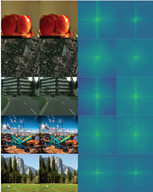
Figure 10: Frequency analysis on additive Gaussian noise with \sigma = 0.02 . We show exemplary images from ap2or , map2sat , citysc , Cezanne , and win2sum categories (in the 1st column), noisy images (in the 2nd column), spectra of original images (in the 3rd column), and spectra of noisy images (in the 4th column).
