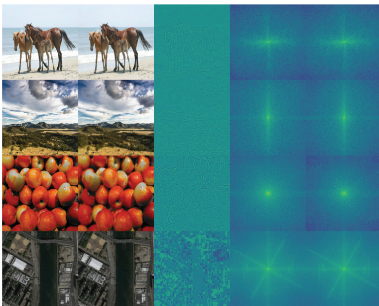
Figure 8: Frequency analysis on JPEG compression (QF = 75). We show exemplary images from hor2zeb , Ukiyoe , ap2or , and map2sat categories (in the 1st column), JPEG compressed images (in the 2nd column), difference maps between original and JPEG compressed images (in the 3rd column), spectra of original images (in the 4th column) and spectra of compressed images (in the 5th column).
