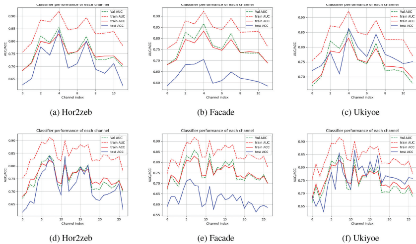
Figure 7: Soft classification performance of six exemplary semantic categories on noisy images ( \sigma = 0.01 ), (a)–(c) uses the 2 \times 2 \times 3 filter bank so that the x -axis has 12 channels, (d)–(f) uses the 3 \times 3 \times 3 filter bank so that the x -axis has 27 channels. Each subfigure shows four performance curves: train set AUC (red dashed line), train set ACC (red line), validation set AUC (green dashed line), and test set ACC (blue line).
