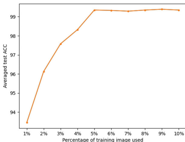
Figure 11: The test accuracy as a function of different percentages of the total training images.
