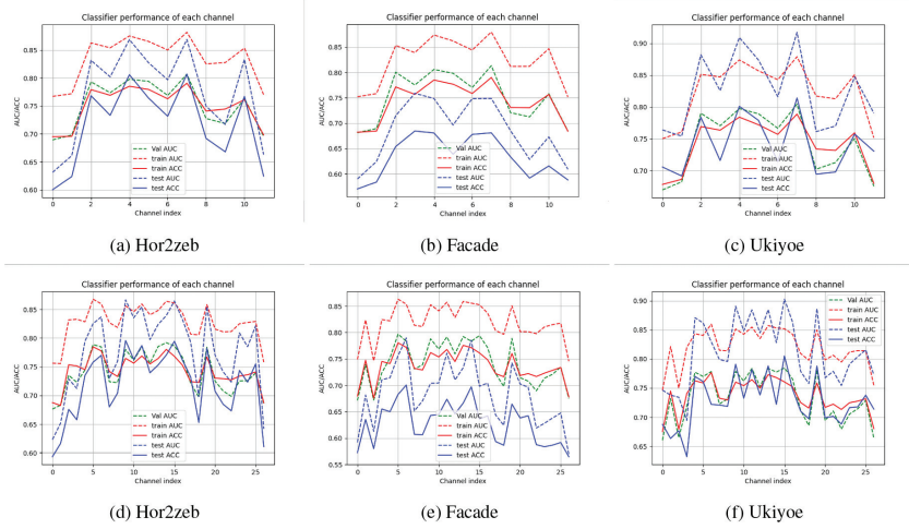
Figure 6: Soft classification performance of exemplary categories on JPEG compressed images (QF=85): For subfigures (a)–(c), the filter size is 2 \times 2 \times 3 (i.e., the number of channels is 12), while for subfigures (d)–(f), the filter size is 3 \times 3 \times 3 (i.e., the number of channels is 27). For each subfigure, we show five performance curves: train set AUC (red dashed line), train set ACC (red line), validation set AUC (green dashed line), test set AUC (blue dashed line), and test set ACC (blue line).
