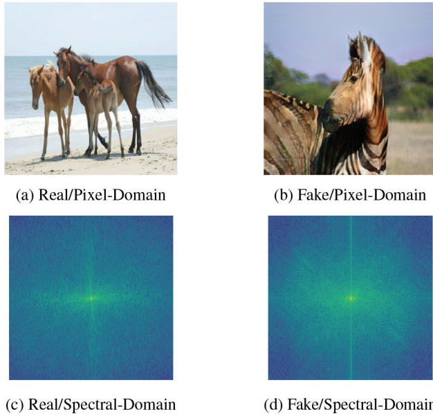
Figure 1: Examples of real/fake image pairs (top) and their associated spectral-domain representation pairs (bottom).
