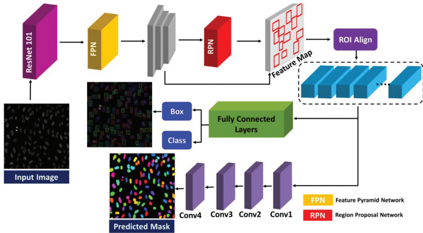
Figure 14: An example Mask RCNN based nuclei segmentation framework from [81] called NucleiNet.
