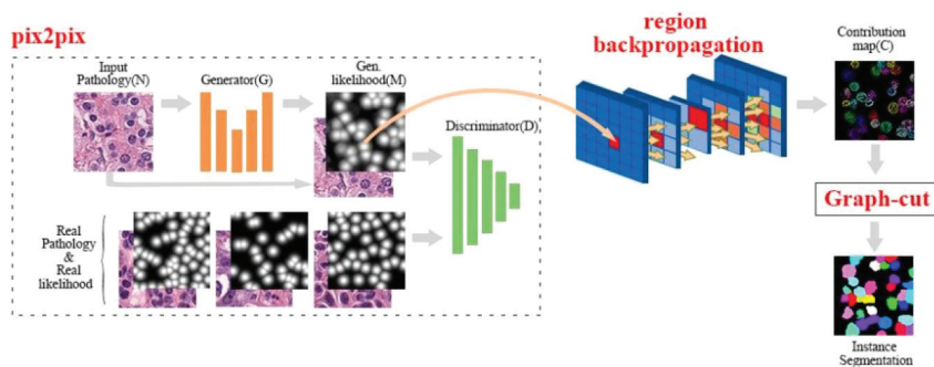
Figure 19: An example framework using GAN to generate a nuclei centroid likelihood map from [37].
