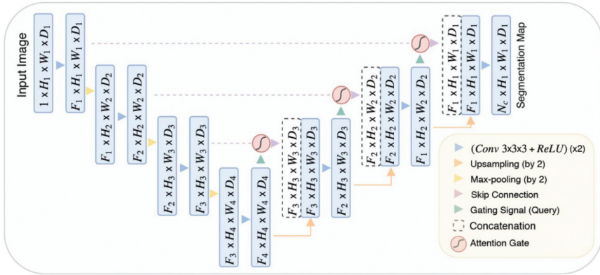
Figure 17: An example of architecture using gated attention for U-Net from [90].
