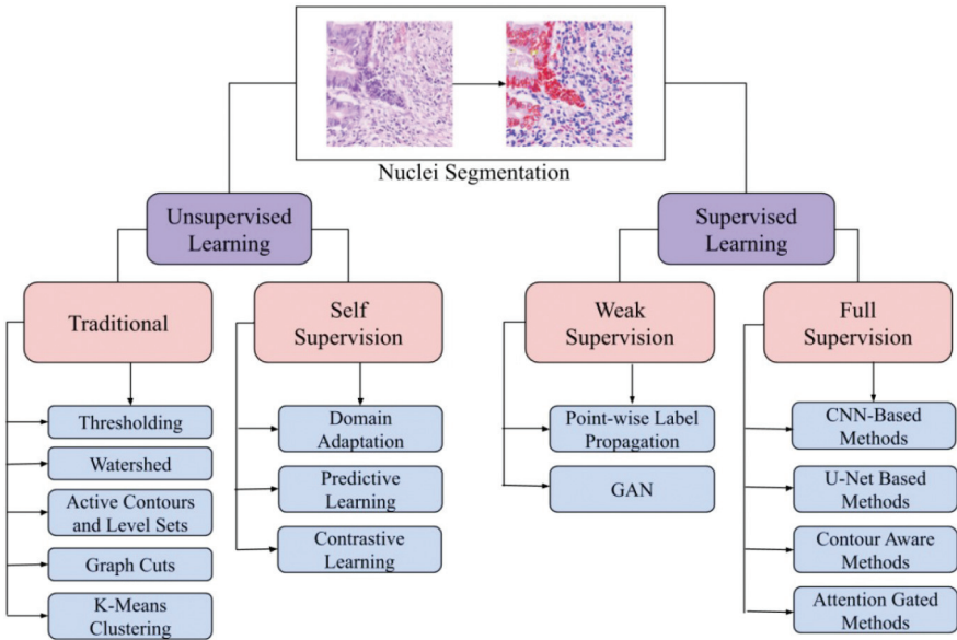
Figure 4: Outline of the existing nuclei segmentation methods.
