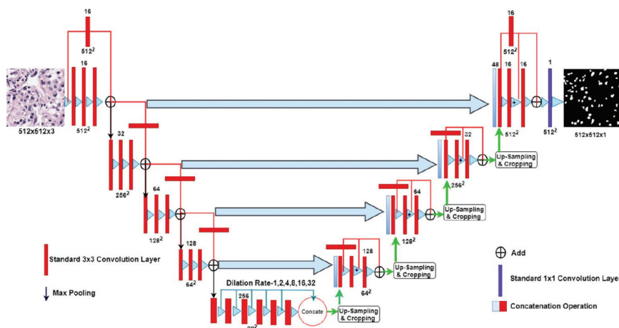
Figure 15: An example U-Net architecture from [11] with an atrous spatial pyramid pooling bottleneck block.
