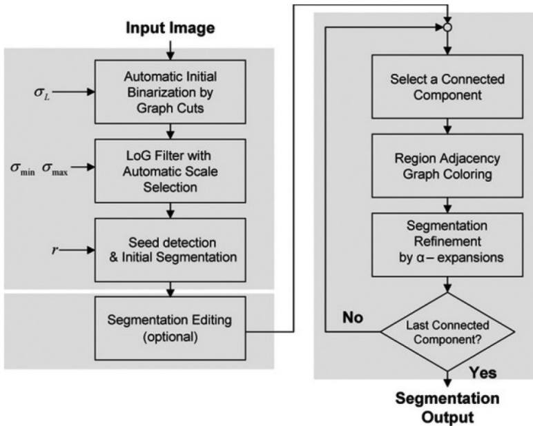
Figure 9: An example graph cuts based pipeline from [45].
