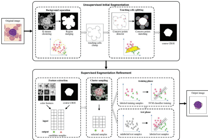
Figure 12: An example image from [108] showing the use of pseudolabels generated from the first stage to train a classifier in the second stage.
