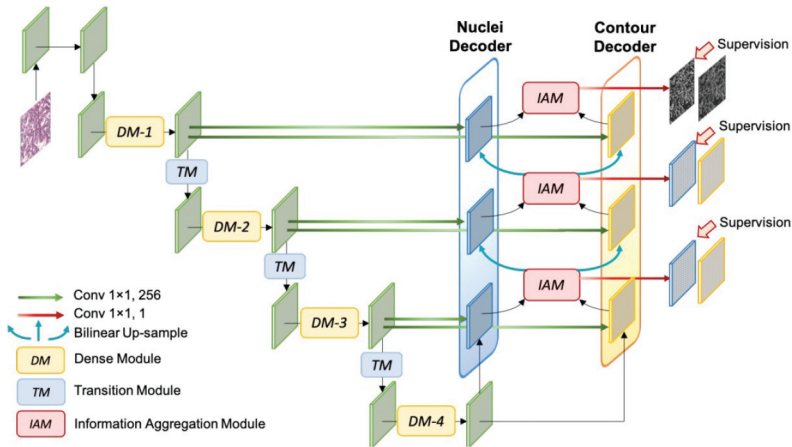
Figure 16: An example of the contour aware CIA-Net from [110] that uses a U-Net architecture with two decoding paths dedicated to nuclei and contour decoding respectively.
