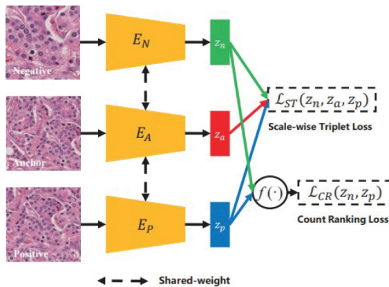
Figure 13: A contrastive learning example from [103] using three different patches generated from an image.
