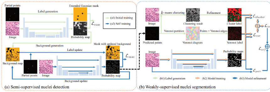
Figure 18: An example of a two stage point wise label propagation from [73].
