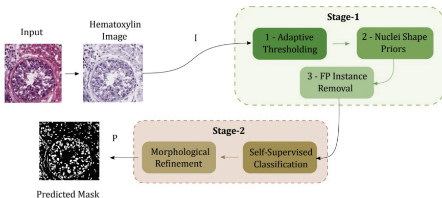
Figure 6: High Performance Unsupervised Nuclei Instance Segmentation (HUNIS) pipeline from [61].
