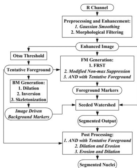
Figure 7: An example marker controlled watershed method from [97] in conjunction with thresholding.
