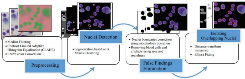
Figure 10: An example K-Means Clustering based pipeline from [101].
