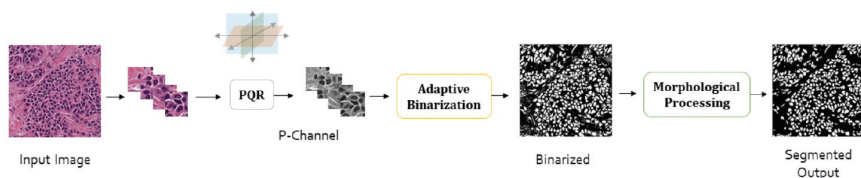
Figure 5: An example thresholding pipeline from [60].
