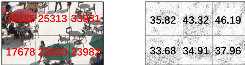
Figure 2: The bit consumption map (left) and SATD distribution of the image (right).
