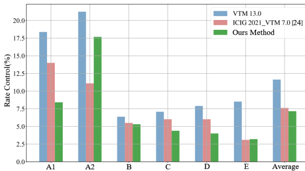
Figure 5: CE performance of the methods.
