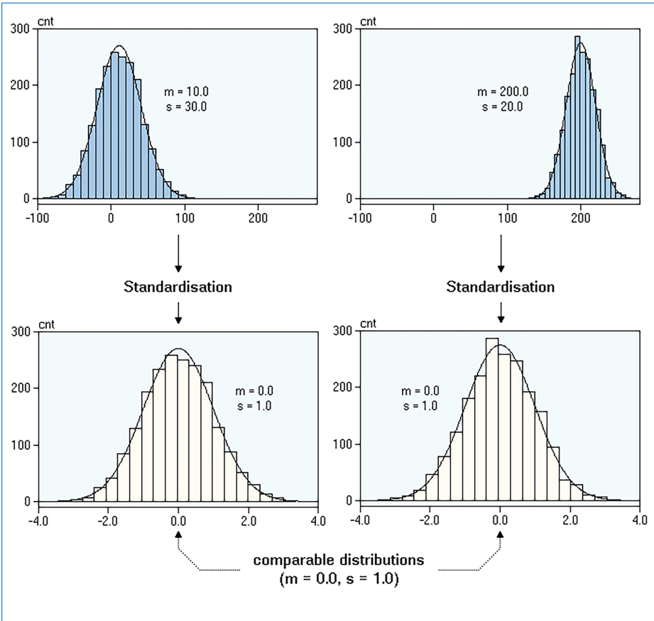
Figure 8.25. Data standardization.
