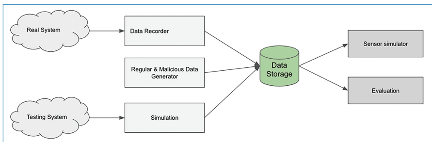
Figure 8.11. DataStorage.
