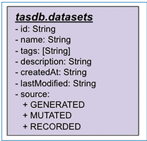
Figure 8.13. Dataset Schema.
