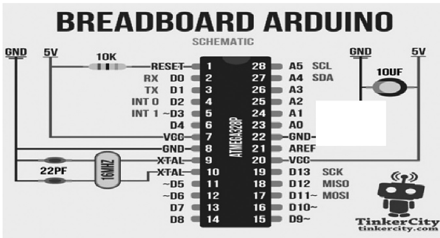
Figure 1. Breadboard Arduino (Syahwil, 2013, p. 24)
