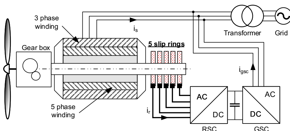
Figure 1. Scheme of the developed novel five- phase DFIG
