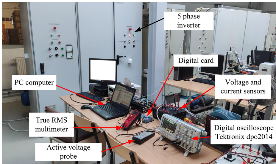
Figure 7. Test bench of the novel five-phase DFIG
