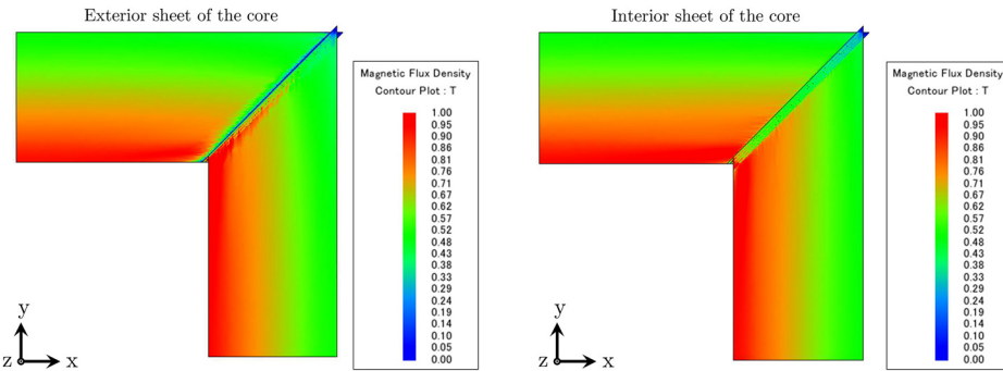
Figure 13. Flux density behavior in the magnetic core for a global flux density of 0.7 T
