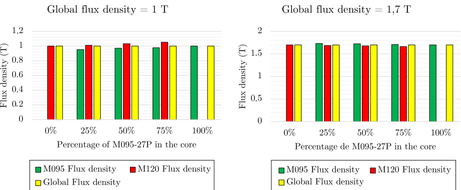
Figure 9. 2D model results of the flux density distribution in the core
