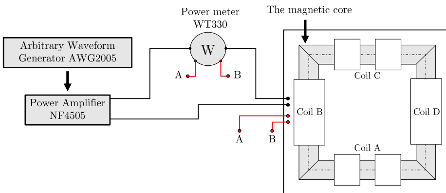
Figure 2. Experimental setup schematic representation
