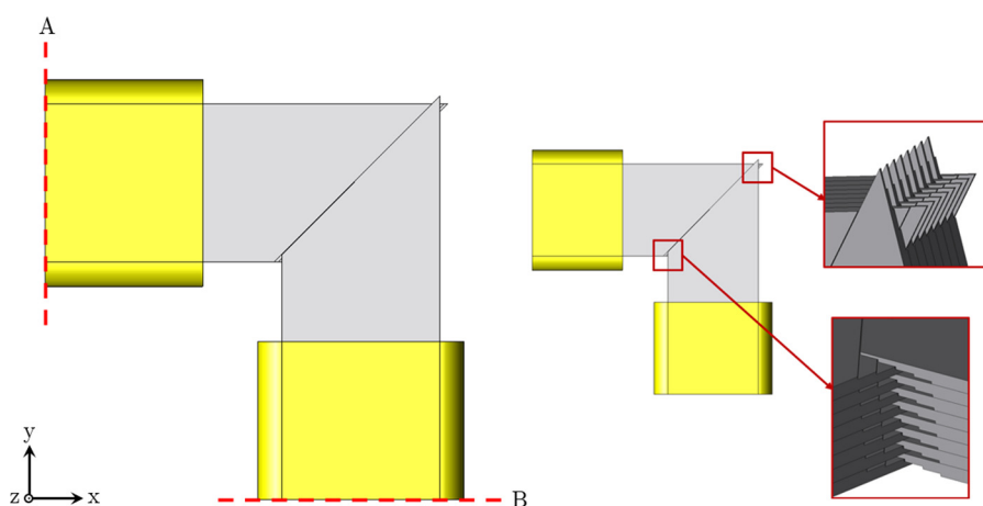
Figure 11. The 3D model of the magnetic core
