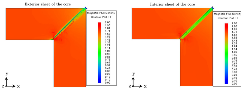
Figure 14. Flux density behavior in the magnetic core for a global flux density of 1.7 T
