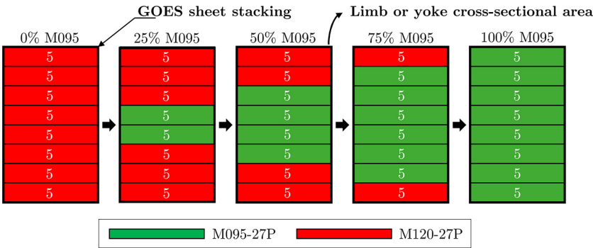
Figure 4. Grade mixing layout in the magnetic core
