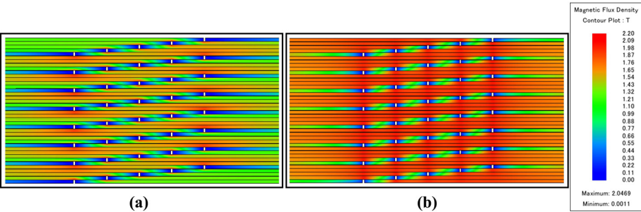
Figure 8. Flux density behavior in the magnetic core joint area
