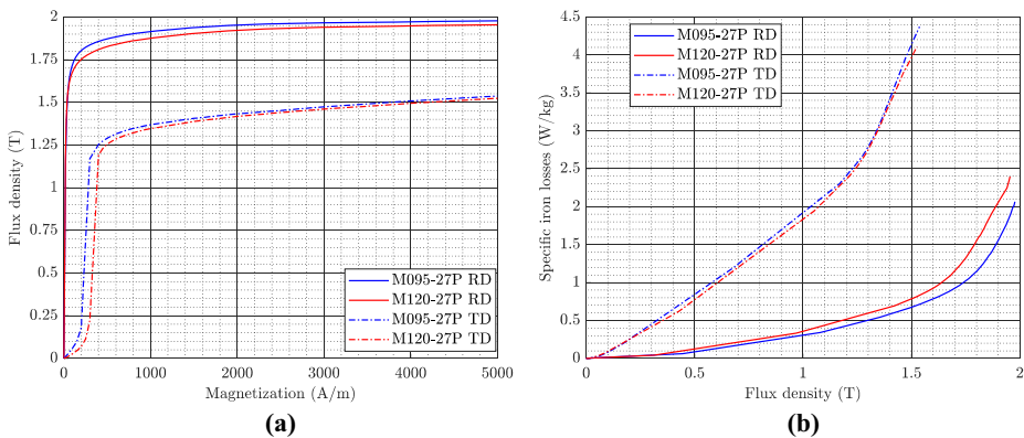
Figure 3. Characteristics of M095-27P and M120-27P at 50 Hz in the RD and TD
