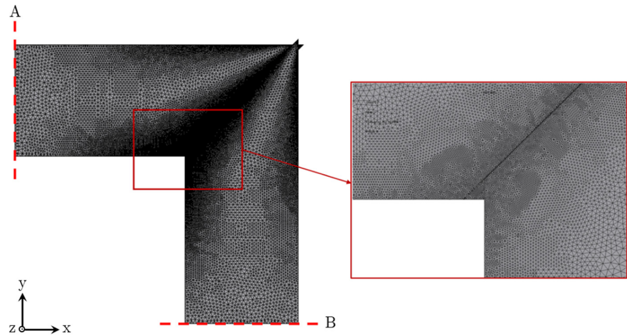
Figure 12. Applied mesh of the 3D model
