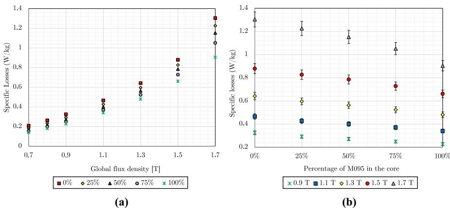
Figure 5. (a) Specific losses variation across the five magnetic cores as a function of the global flux density and (b) variation of the specific losses as a function of the flux density and the percentage of M095-27P in the core
