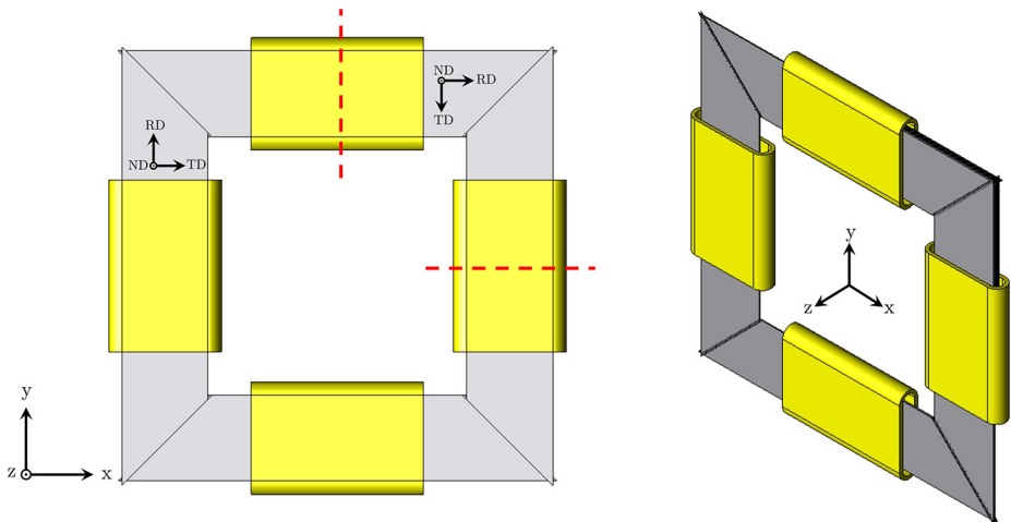
Figure 6. The single-phase magnetic core FEA model
