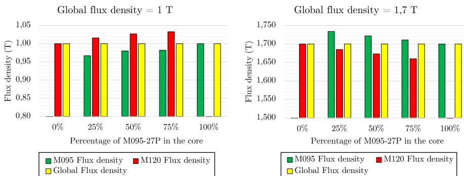
Figure 15. 3D model results of the flux density distribution in the core
