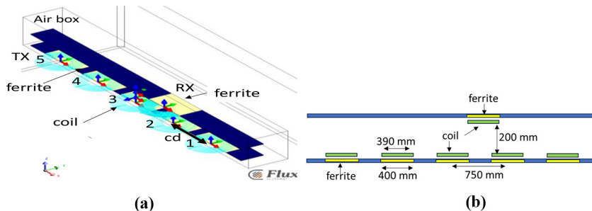
Figure 1. Layout of the DWPT system model considered for the FEA
