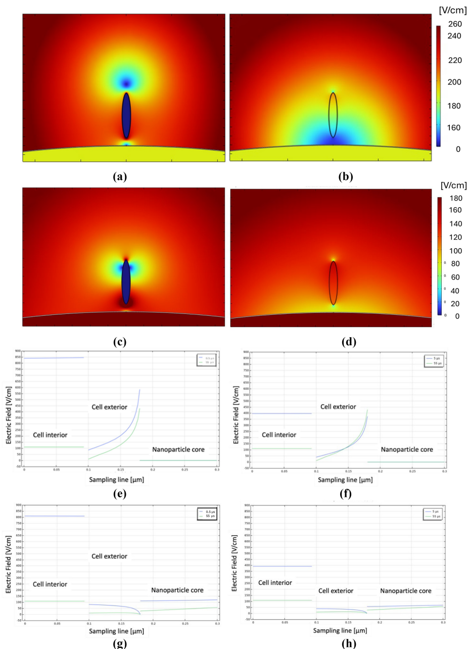
Figure 5. Electric field strength for (a)–(c) gold and (b)–(d) dielectric nanoparticle vertically-oriented in position P_0 at (a) and (b) 55 \mu\text{s} and at (c) and (d) t = \tau/2 considering a pulse with a rise time of 1 \mu\text{s} . Electric field along L_c for (e) and (f) gold and (g) and (h) dielectric nanoparticle for a pulse rise time of (e)–(g) 1 \mu\text{s} and (f)–(h) 10 \mu\text{s}
