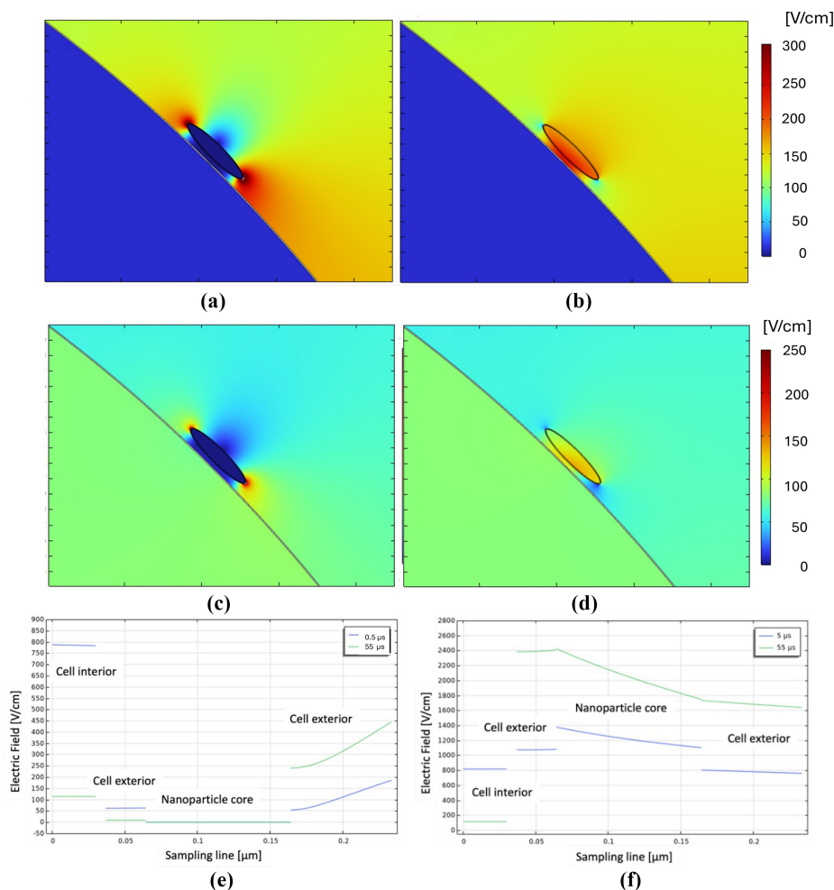
Figure 6. Electric field strength for (a)–(c) gold and (b)–(d) dielectric nanoparticle in position P_{45} at (a) and (b) 55\mu\text{s} and at (c) and (d) t_r/2 considering a pulse with a rise time of 1\mu\text{s}
