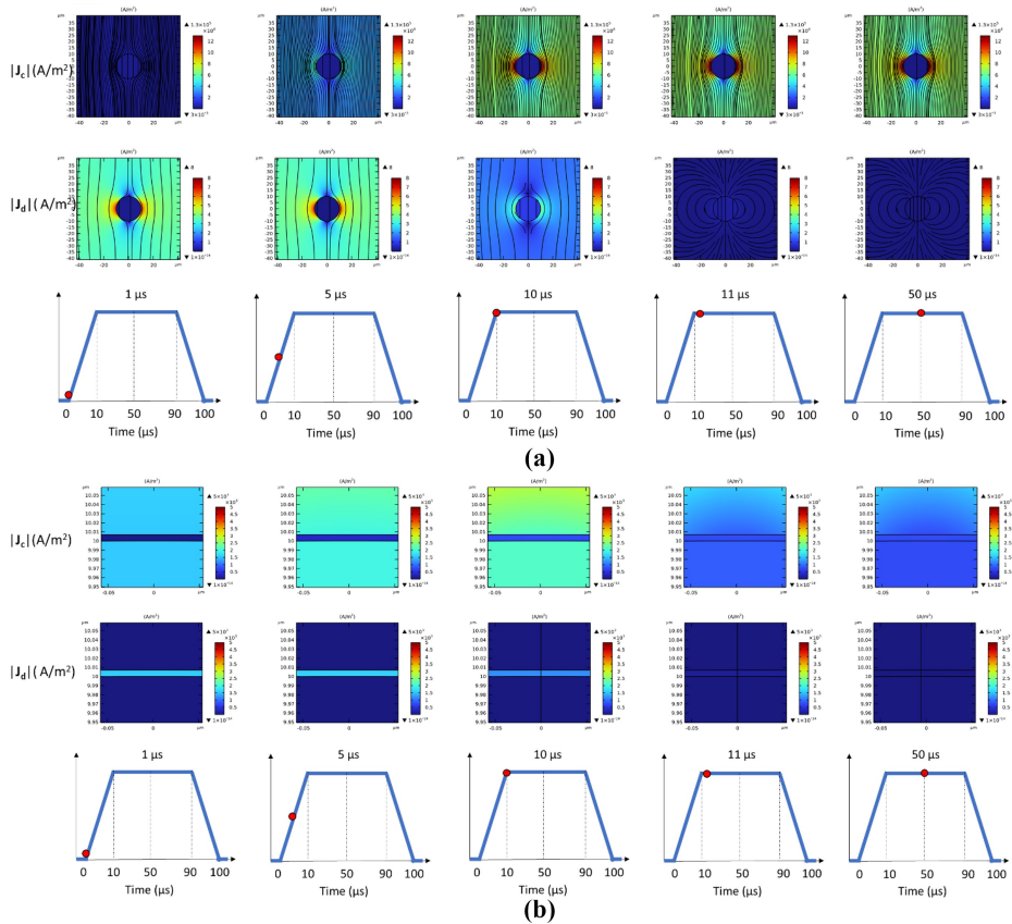
Figure 2. Evaluation of the conduction current (upper line), |J_c| , and displacement current density (middle line), |J_d| , at 1, 5, 10, 11 and 50 \mu\text{s} in (a) the entire domain and (b) on the membrane (the rectangular strip is the membrane)
