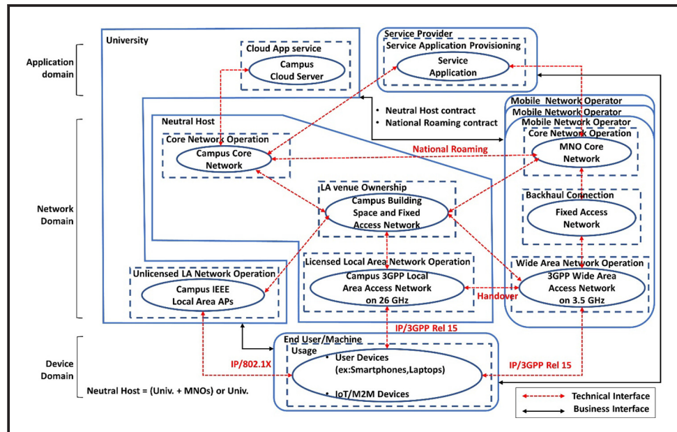
Figure 10 Neutral host-driven VNC (national roaming based)
