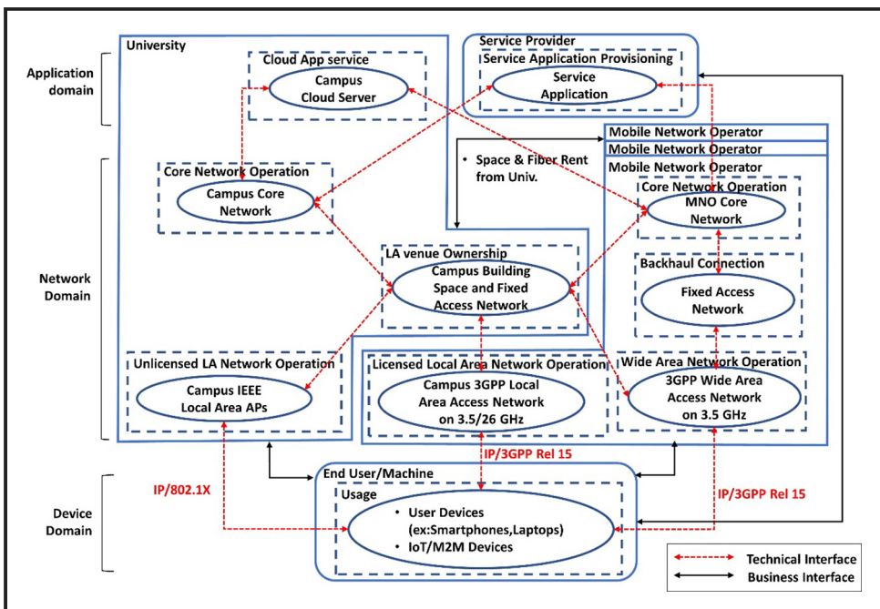
Figure 8 Multi-MNO-driven VNC
