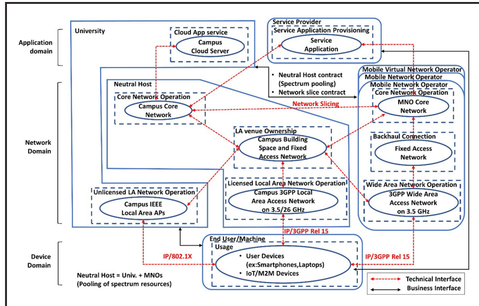
Figure 9 Neutral host-driven VNC (network slicing based)
