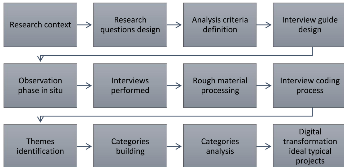
Figure 1. Methodology flowchart.
