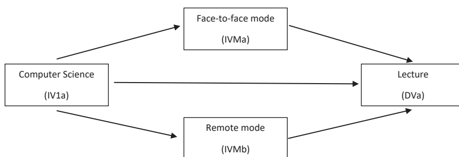
Figure 1. GML mediation model using Computer science (IV1a) and Lecture (DVa) as an example
