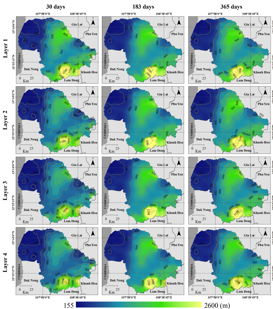
Figure 4. Head water at four layers in each simulation period
