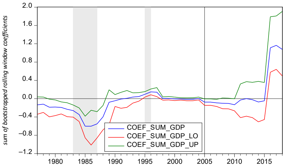
Figure 2. Bootstrap estimates of the sum of the rolling window coefficients for the impact of GDP on DEF
