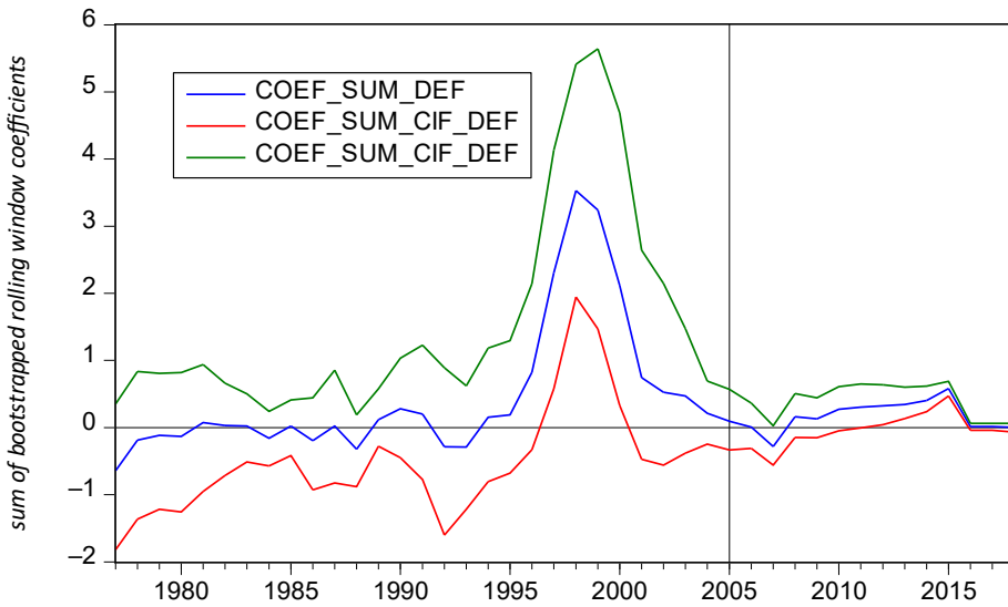
Figure 4. Bootstrap estimates of the sum of the rolling window coefficients for the impact of DEF on GDP
