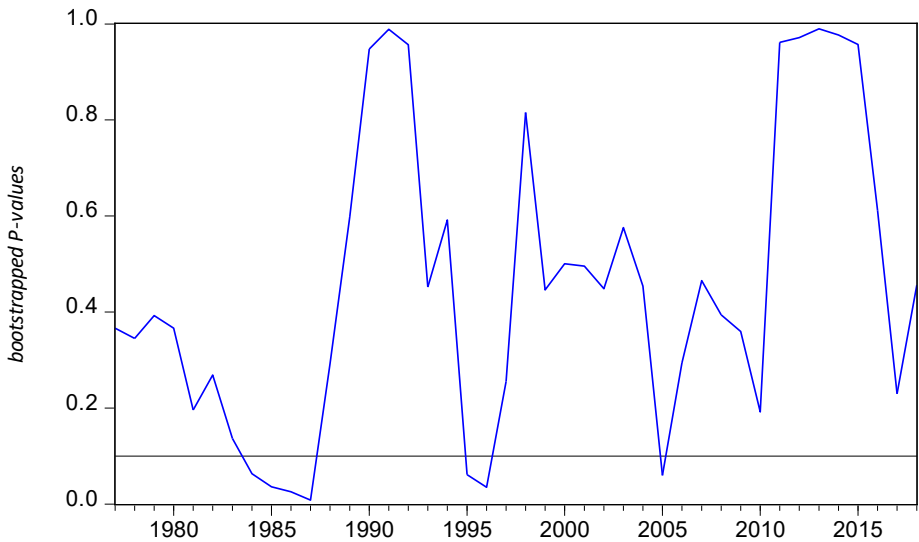
Figure 1. Bootstrapped probability values for testing the null hypothesis that GDP does not Granger cause DEF
