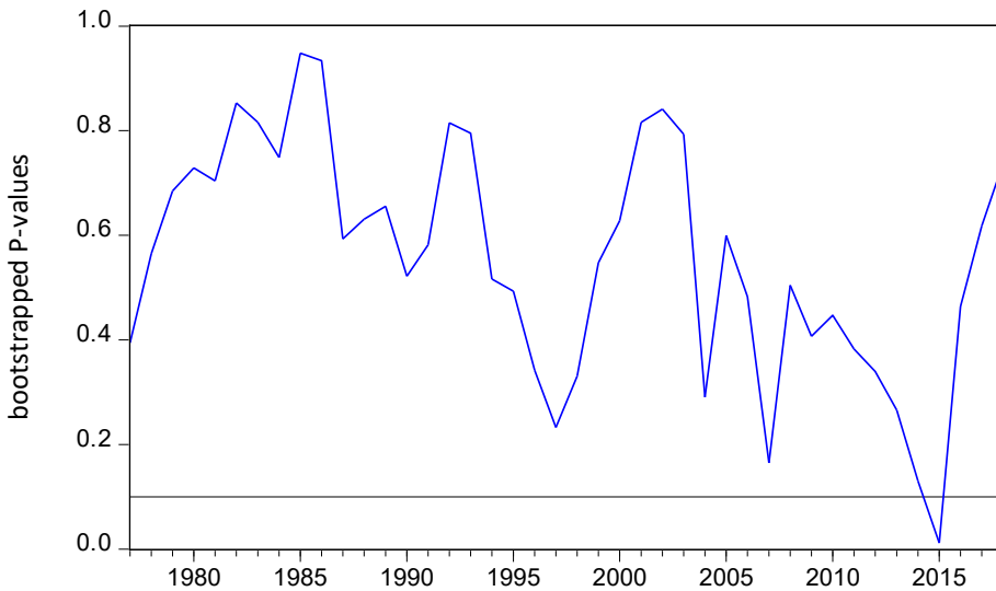
Figure 3. Bootstrapped probability values for testing the null hypothesis that DEF does not Granger cause GDP
