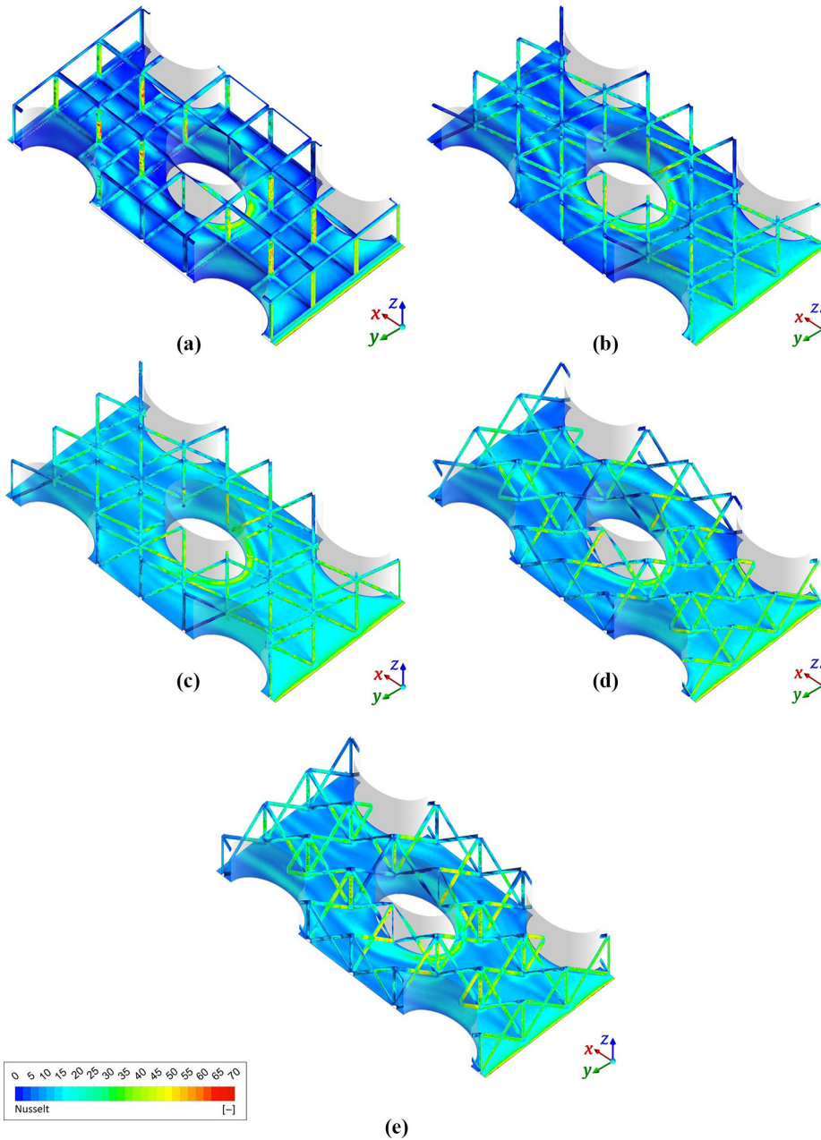
Figure 15. Distribution of local Nusselt number on the ligaments and inner surface of the lower fin, for PCLs at \varepsilon = 98\% , Re_{D_h} = 3000
