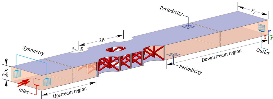
Figure 4. 3 D schematic representation of the geometric details of a trussed FETHX with PCL structure and BCs for the CD
