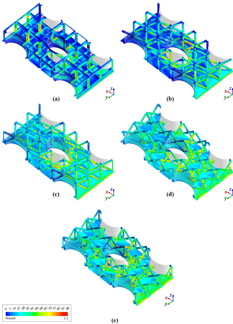
Figure 14. Distribution of local Nusselt number on the ligaments and inner surface of the lower fin, for PCLs at \varepsilon = 92\% , Re_{D_h} = 3000
