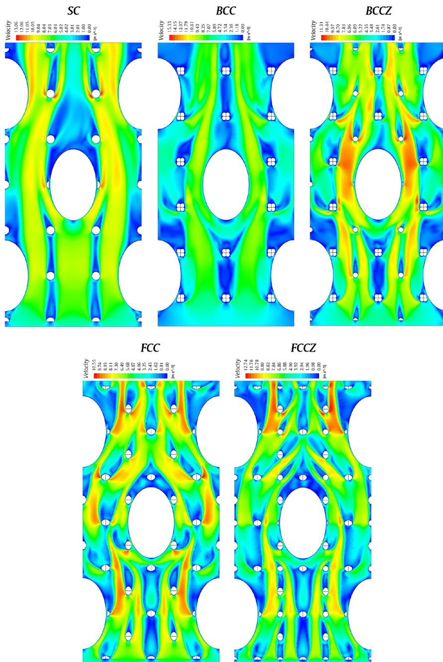
Figure 12. Local distribution of the velocity (in the middle xy -plane) for PCLs at \varepsilon = 92\% , Re_{D_h} = 3000
