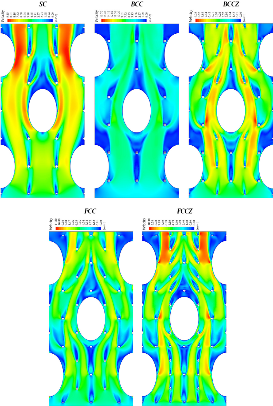
Figure 13. Local distribution of the velocity (in the middle xy -plane) for PCLs at \varepsilon = 98\% , Re_{D_h} = 3000
