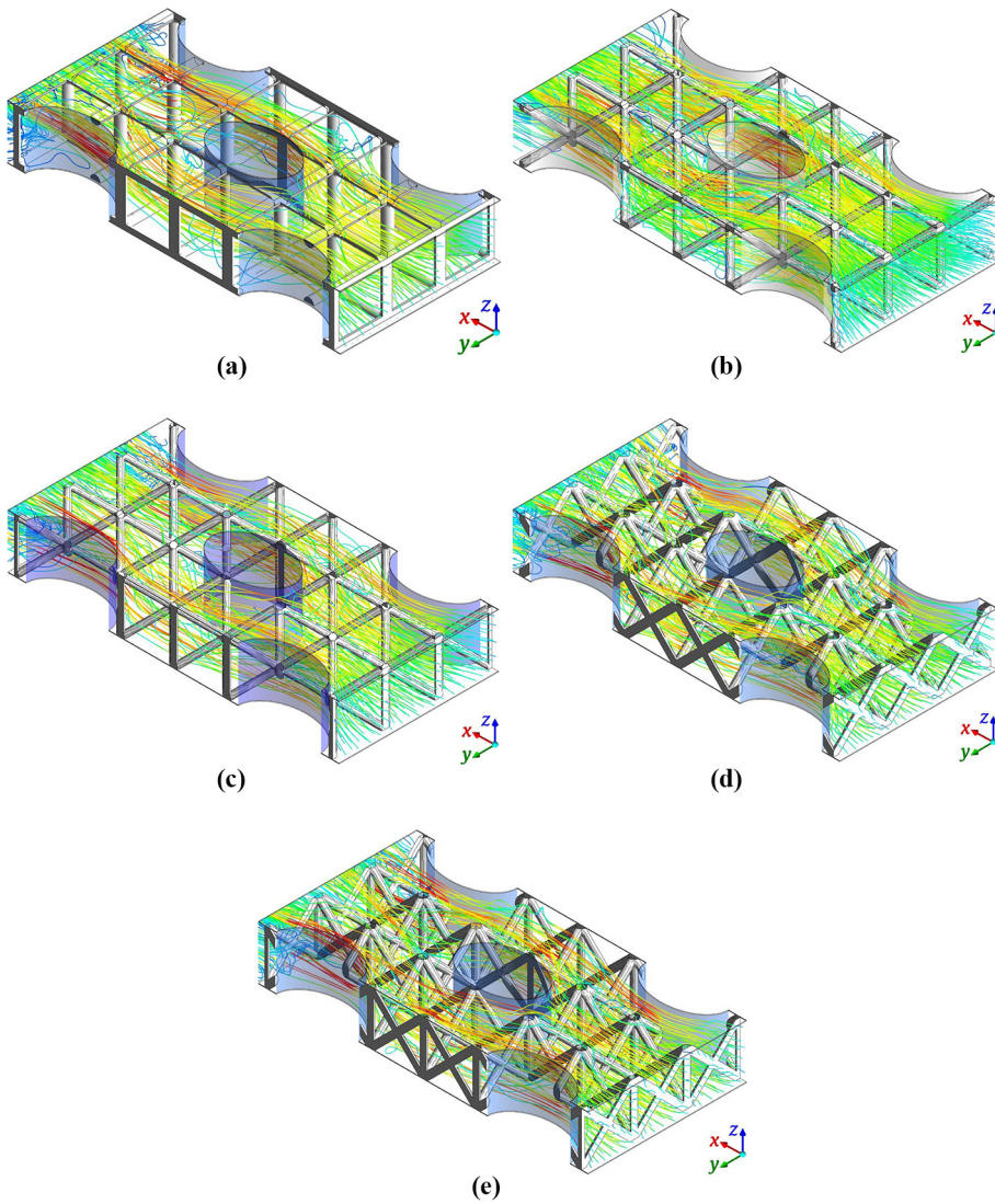
Figure 8. Comparison of flow patterns indicated by three-dimensional trajectories close to trussed fin surfaces induced by PCL structures with \varepsilon = 92\% , at Re_{D_h} = 3000
