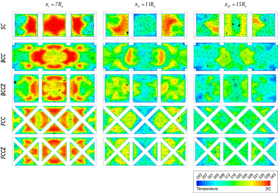
Figure 9. Streamlines and temperature contours in transverse planes at \varepsilon = 92\% , Re_{D_h} = 3000
