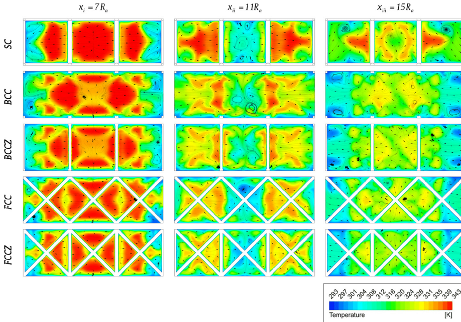
Figure 10. Streamlines and temperature contours in transverse planes at \varepsilon = 98\% , Re_{D_h} = 3000
