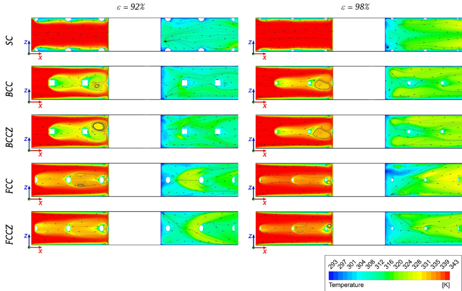
Figure 11. Velocity streamlines and temperature contours in longitudinal central plane at y = P_t/2 , Re_{D_h} = 3000
