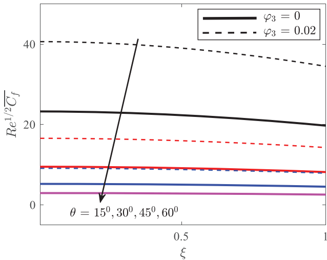
Figure 16. Impact of yaw angle ( \theta ) and third component of the ternary hybrid nanofluent ( \varphi_3 ) on the spanwise skin-friction coefficient
