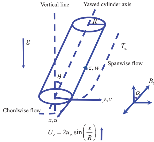
Figure 1. Flow illustration
