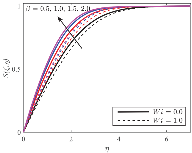
Figure 4. Impact of Casson parameter ( \beta ) and Williamson parameter ( Wi ) on the spanwise velocity profile
