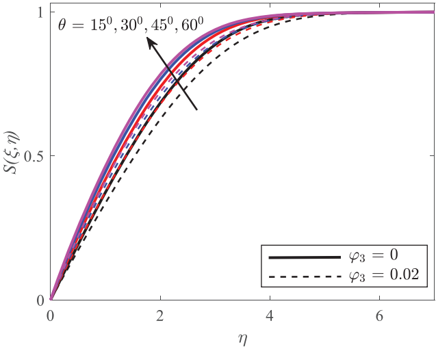
Figure 14. Impact of yaw angle ( \theta ) and third component of the ternary hybrid nanofluid ( \varphi_3 ) on the spanwise velocity profile
