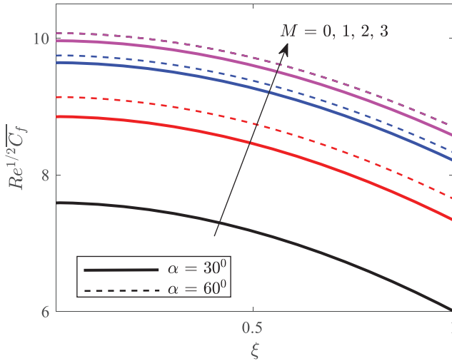
Figure 11. Impact of inclined magnetic field parameter ( m ) and angle of inclination ( \alpha ) of the magnetic field on the spanwise skin-friction coefficient
