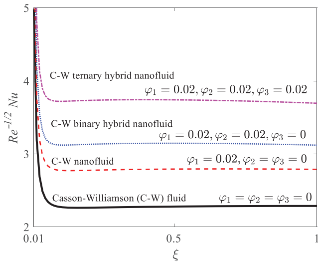
Figure 17. Energy transfer rate of different fluids (base fluid, nanofluent, bi-component and tri-component hybrid nanofluids)
