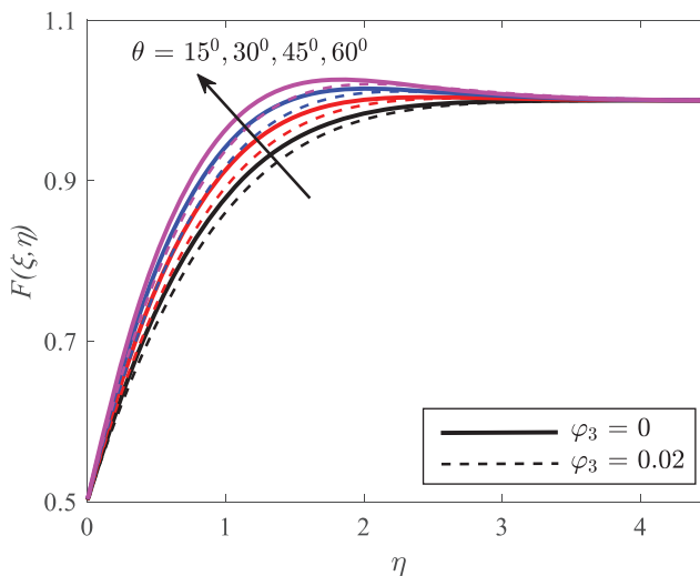
Figure 13. Impact of yaw angle ( \theta ) and third component of the ternary hybrid nanofluid ( \varphi_3 ) on the Chordwise velocity profile
