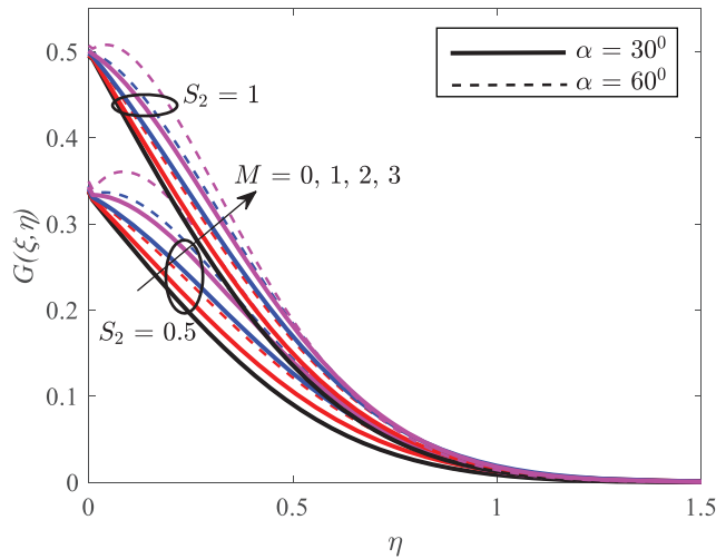
Figure 9. Impact of thermal jump ( S_2 ), inclined magnetic field parameter ( m ) and angle of inclination ( \alpha ) of the magnetic field on the temperature profile
