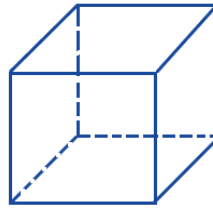
Hexahedron ( s = 3.7221 )
