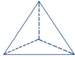
Tetrahedron ( s = 4.0613 )
