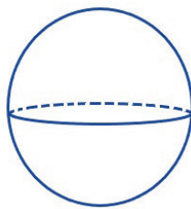
Sphere ( s = 3.0 )
