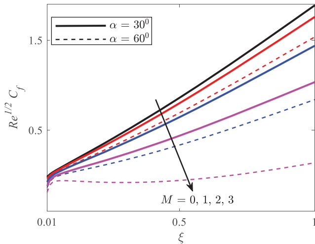
Figure 10. Impact of inclined magnetic field parameter ( m ) and angle of inclination ( \alpha ) of the magnetic field on the chordwise skin-friction coefficient
