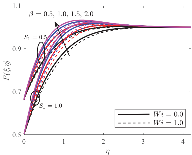
Figure 3. Impact of velocity slip ( S_1 ), Casson parameter ( \beta ) and Williamson parameter ( Wi ) on the chordwise velocity profile
