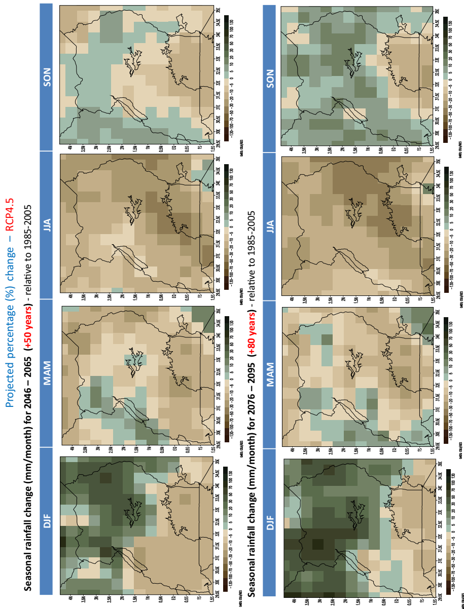
Figure 4. Projected percentage change of seasonal rainfall change for 2046 -2065 relative to 1985- 2005 of the RCP4.5 scenario
