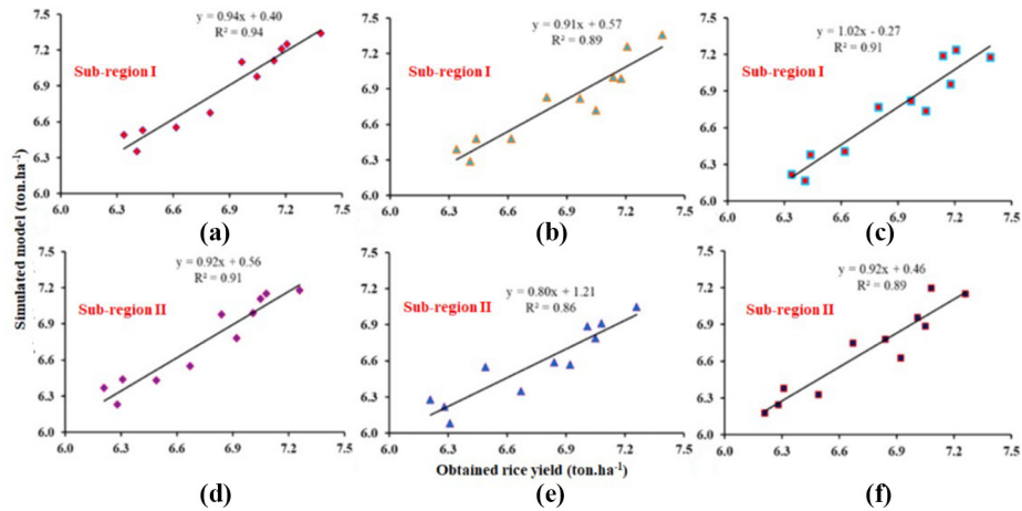
Figure 3. Results of model calibration based on the simulated and observed yield of a) spring, b) summer and c) autumn– winter planting seasons in subregion I; and d) spring, e) summer and f) autumn–winter planting seasons in subregion II
