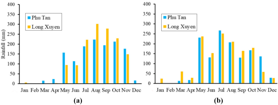
Figure 2. Precipitation data for a) model calibration using 2000–2010 data and b) model validation using 2011–2018 data
