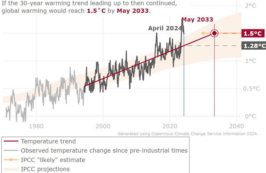
Figure 4. Linear trend projection of 30-year (1994–2033) temperatures over the next decade
