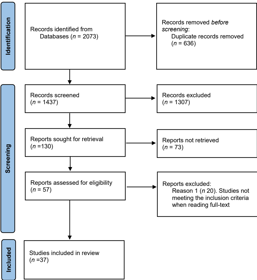
Figure 1. The PRISMA 2020 flow diagram of article selection process
