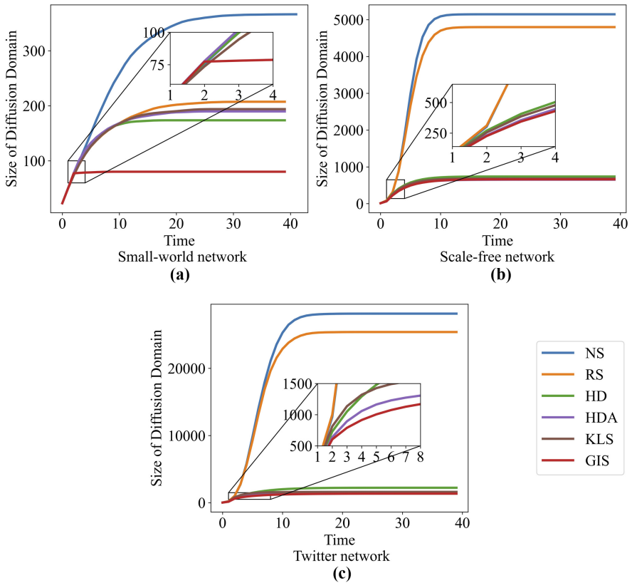
Figure 4. Network immunity
