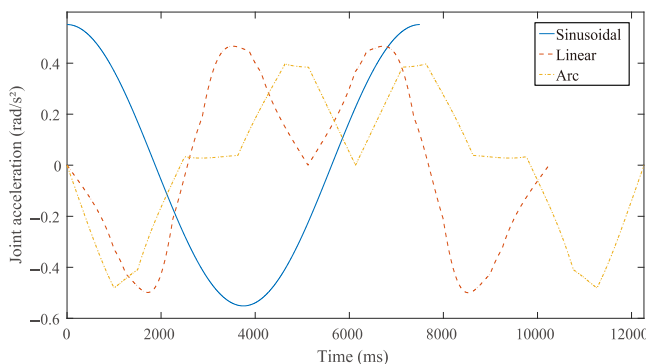
Figure 10 The target acceleration of Joint 1 when the robot runs the test trajectory
