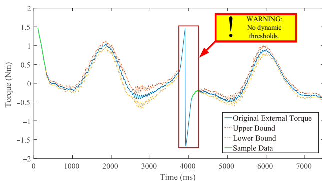
Figure 3 The defect of the collision detection method based only on TSA
