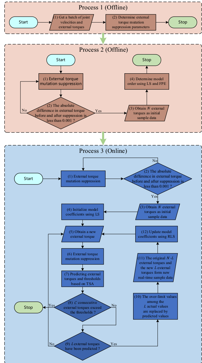
Figure 7 Flow chart of the method proposed in this paper
