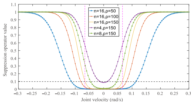
Figure 6 Suppression operator O_{sp} under different \rho and n
