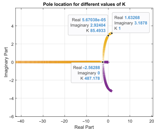
Figure 4 Location of roots of the characteristic equation in equation (4) for different values of K_r and B_r with M_r = 10
