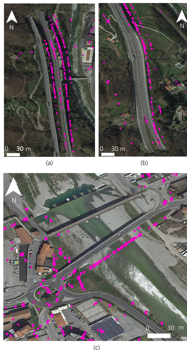
Figure 9. Examples of PS geolocation errors for (a) a motorway viaduct, (b) a motorway segment and (c) a motorway bridge in the Liguria region of Italy. Each dot corresponds to a PS. A full-colour version of this figure can be found on the ICE Virtual Library ( www.icevirtuallibrary.com )
