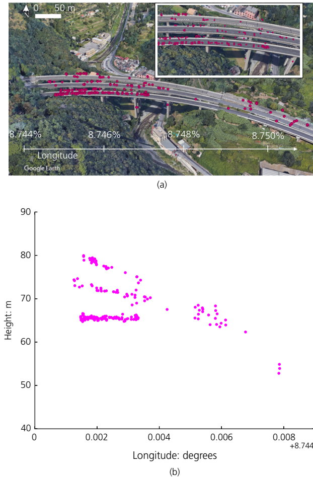
Figure 5. PSs identified on a motorway viaduct in Genoa, Italy: (a) 3D view of PSs on the viaduct from Google Earth; (b) estimated longitudes and elevations of the PSs detected on the asset. Each dot indicates a PS. The PSs were obtained by processing 130 COSMO-SkyMed ascending images from 2011 to 2018 using the software package Sarproz (Perissin et al. , 2011). Map data © 2020 Google Earth Pro
