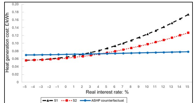
Figure 6. Real price of heat (£/kWh) expressed in £2024 against the real interest rate. Calculated by equating NPV to zero
