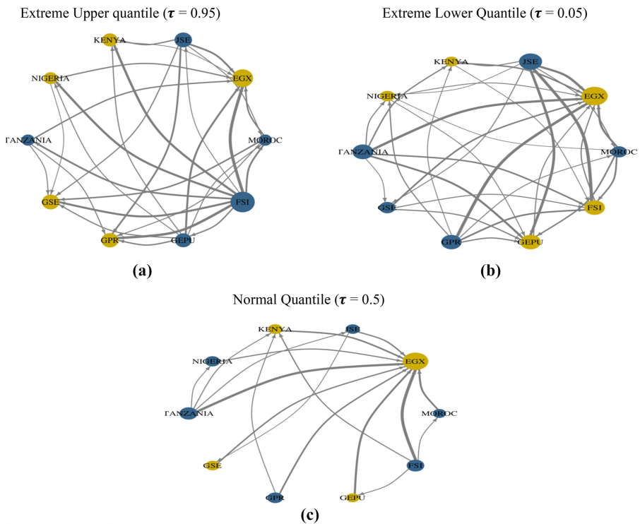
Figure 1. Returns connectedness network plot
