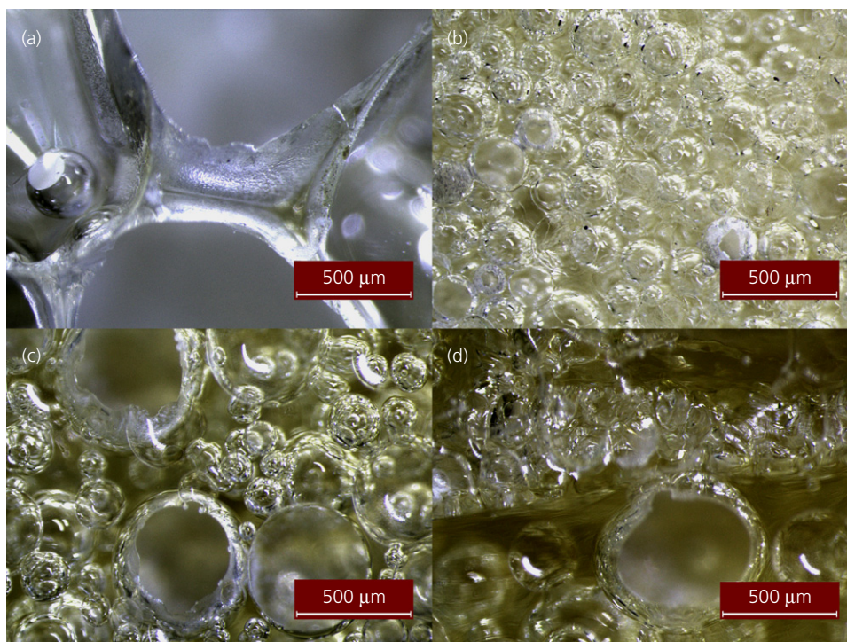
Figure 9. Stereo optical microscopy images taken at 5 \times : (a) LD40 cut-edge, (b) Reproc cell 300 cut-edge, (c) Reproc cell 500 cut-edge, (d) Reproc cell 500 interface
