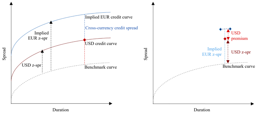
Figure 2. Stylised representation of the cross-currency credit spread
