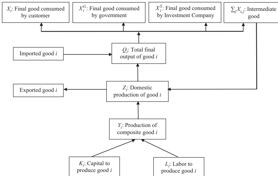
Figure 2. Tree structure of production decision
