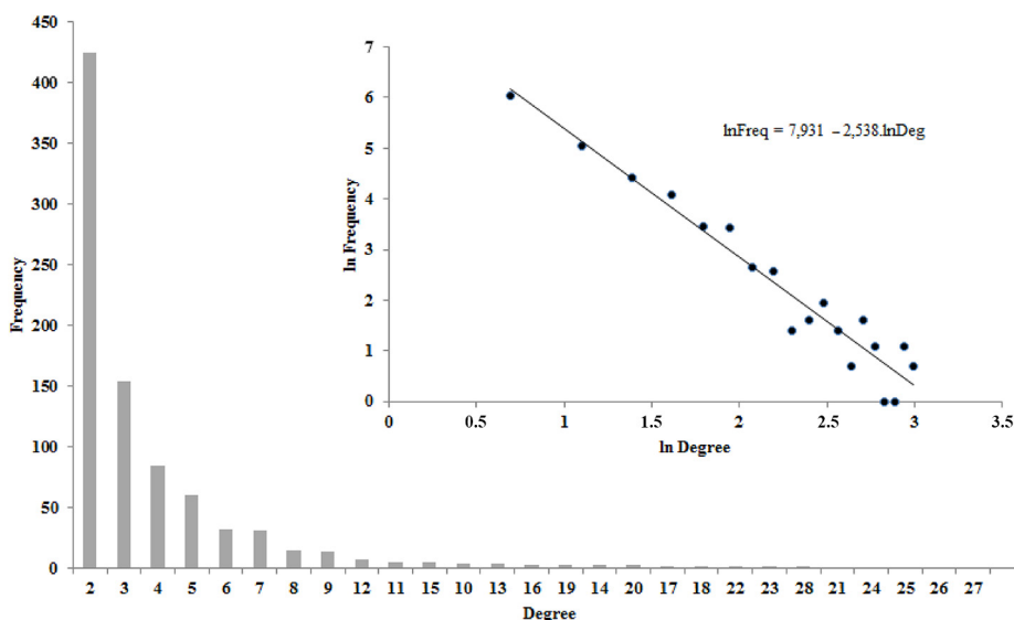
Figure 3. Frequency of degrees and log-log representation
