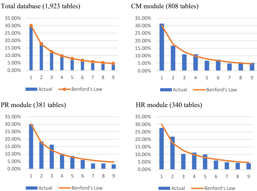
Figure 1. Actual and Benford's law expected frequency distributions
