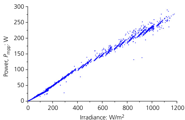
Figure 6. Maximum power point, P_{mpp} (W), plotted against irradiance ( W/m^2 ) for HIT
