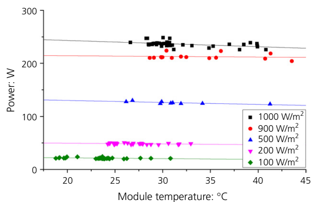
Figure 5. Temperature effect (°C) on the output power (W) of the HIT module
