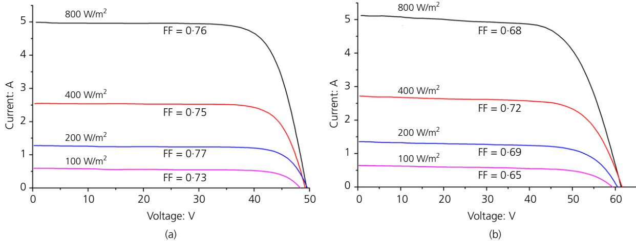
Figure 3. I - V curves at different irradiance levels for: (a) the HIT panel and (b) the p-Si panels
