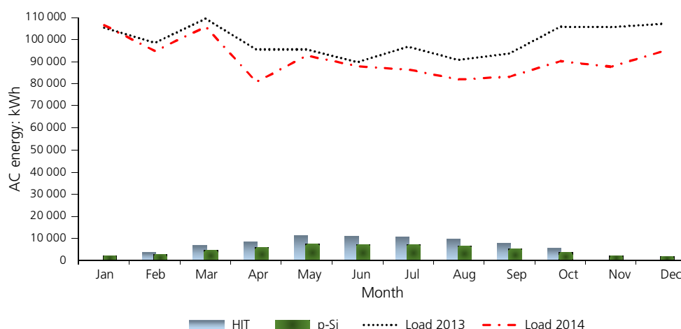
Figure 7. Energy balance, AC energy load (2013 and 2014) and potential PV energy generation
