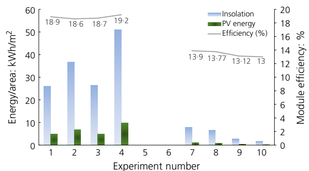
Figure 4. Insolation, PV energy generation and module efficiency against experiment number
