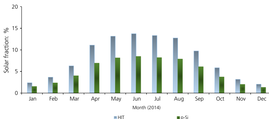
Figure 8. Monthly solar fraction for HIT and p-Si PV technologies
