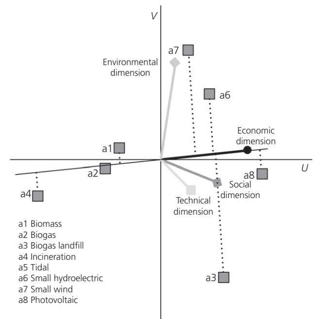
Figure 5. Gaia diagram, DRM case
