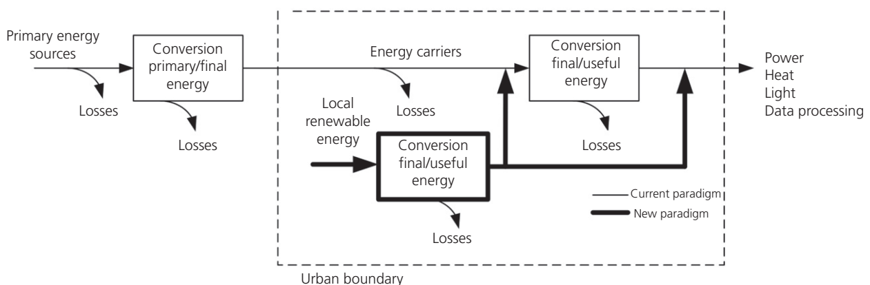
Figure 1. The current and suggested energy models (courtesy: WIT Press)
