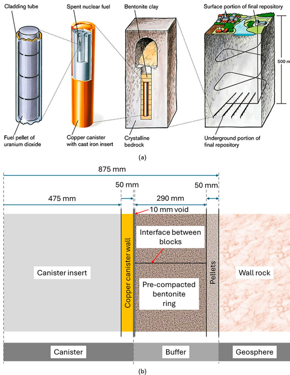
Figure 1. The KBS-3 disposal concept. (a) Diagram of the disposal system from fuel pellet up to the deep geological repository. (b) Cross-section sketch through the Läsit deposition hole showing the canister, engineered void, pre-compacted bentonite ring, pellets, and wall rock. The bentonite ring and pellets make up the buffer, isolating the canister from the geosphere
