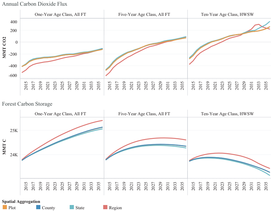
Figure 6: Annual CO 2 flux (where negative value represents sequestration) and carbon stock (where positive value represents carbon stored in forests) comparison across different aggregation sources.
