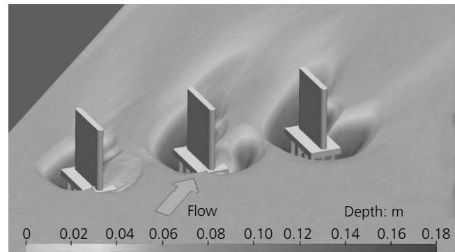
Figure 1. Three-dimensional scour bathymetry for triple complex piers
