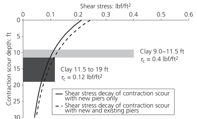
Figure 15. Shear stress decay of contraction scour using SRH-2D results. 1 ft = 0.305 m; 1 lbf/ft 2 = 47.9 Pa
