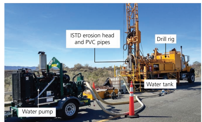
Figure 5. Field set-up of the ISTD. PVC, poly(vinyl chloride)
