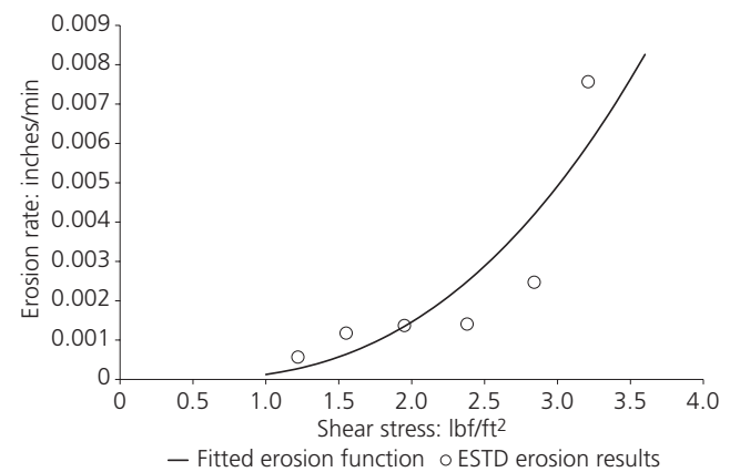
Figure 13. ESTD erosion test results for clay from 9.0 to 11.5 ft (2.7 to 3.5 m). 1 inch = 25.4 mm; 1 lbf/ft 2 = 47.9 Pa
