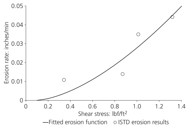
Figure 12. ISTD erosion test results for clay from 10.3 to 11.8 ft (3.1 to 3.6 m). 1 inch = 25.4 mm; 1 lbf/ft 2 = 47.9 Pa
