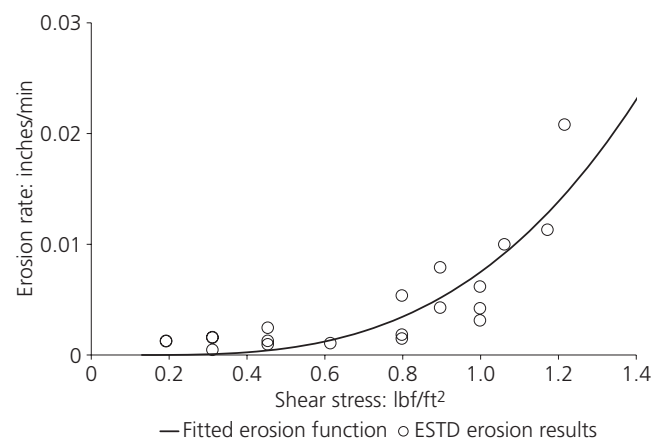
Figure 14. ESTD erosion test results for clay from 11.5 to 19.0 ft (3.5 to 5.8 m). 1 inch = 25.4 mm; 1 lbf/ft 2 = 47.9 Pa
