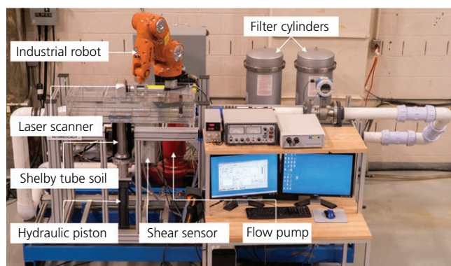
Figure 4. Layout of the ESTD
