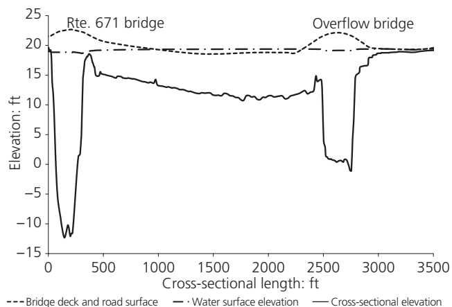
Figure 9. Water surface elevation 100 ft (30 m) upstream of both bridges. 1 ft = 0.305 m
