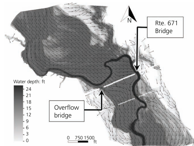
Figure 8. SRH-2D flow depth and velocity vectors for the 100-year flood event. 1 ft = 0.305 m
