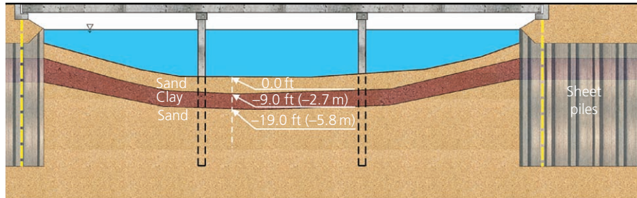
Figure 11. Approximate soil strata at the foundation of the Rte. 671 Bridge
