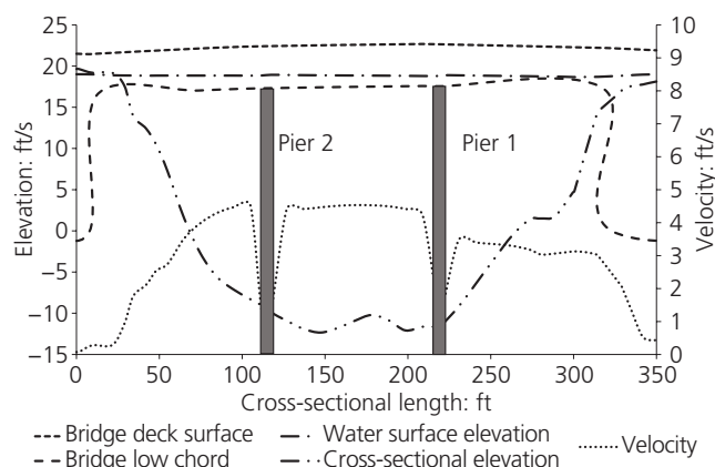
Figure 10. Flow parameters 100 ft (30 m) upstream of the Rte. 671 Bridge. 1 ft = 0.305 m
