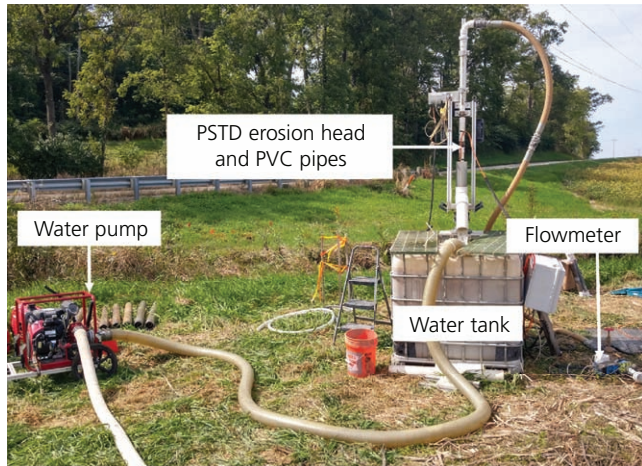
Figure 7. Field set-up of the PSTD. PVC, poly(vinyl chloride)
