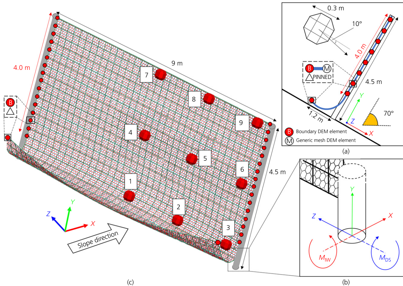
Figure 1. DEM simulation of rockfall fence protection showing different boulder impact positions that were analysed (Previtali et al. , 2021: p. 500)
