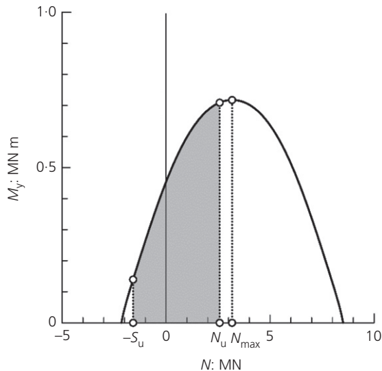
Fig. 6. N - M_y interaction diagram of circular reinforced-concrete cross-section in case of end-bearing piles
